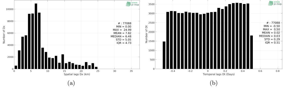
Figure 5: Histograms of the spatial (a) and temporal (b) lags between the time of the TSG (SAMOS) measurements and the date of the corresponding SMOS SSS L2 v662 (ESA) SSS product.
