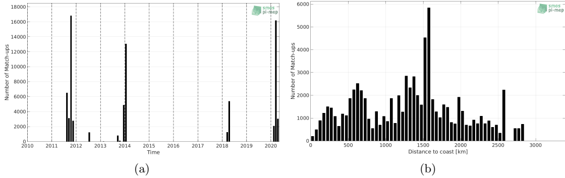
Figure 1: Number of match-ups between TSG (SAMOS) and SMOS SSS L2 v662 (ESA) SSS as a function of time (a) and as function of the distance to coast (b) over the South Atlantic Ocean Pi-MEP region and for the full satellite product period.
