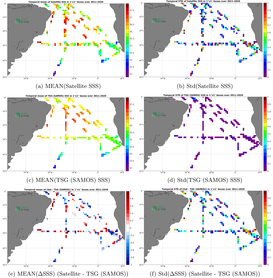
Figure 6: Temporal mean (left) and Std (right) of SSS from SMOS SSS L2 v662 (ESA) (top), TSG (SAMOS) (middle), and of \Delta SSS (Satellite - TSG (SAMOS)). Only match-up pairs are used to generate these maps.
