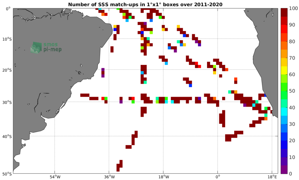
Figure 4: Number of SSS match-ups between TSG (SAMOS) SSS and the SMOS SSS L2 v662 (ESA) SSS product for the South Atlantic Ocean Pi-MEP region over 1°x1° boxes and for the full satellite product period.
