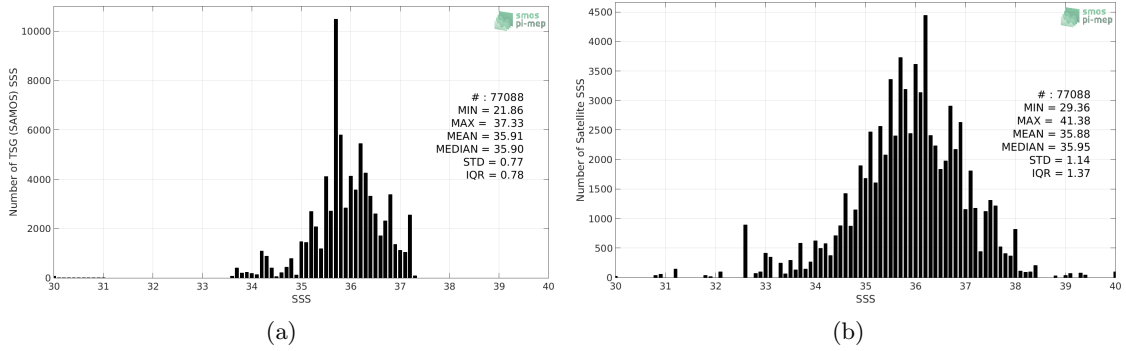
Figure 2: Histograms of SSS from TSG (SAMOS) (a) and SMOS SSS L2 v662 (ESA) (b) considering all match-up pairs per bins of 0.1 over the South Atlantic Ocean Pi-MEP region and for the full satellite product period.
