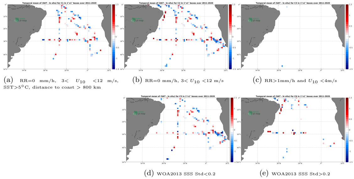
Figure 12: Temporal mean gridded over spatial boxes of size 1^\circ \times 1^\circ of \Delta SSS (SMOS SSS L2 v662 (ESA) - TSG (SAMOS)) for 5 different subdatasets corresponding to: RR=0 mm/h, 3 < U_{10} < 12 m/s, SST > 5^\circ C , distance to coast > 800 km (a), RR=0 mm/h, 3 < U_{10} < 12 m/s (b), RR > 1 mm/h and U_{10} < 4 m/s (c), WOA2013 SSS Std < 0.2 (d), WOA2013 SSS Std > 0.2 (e).
