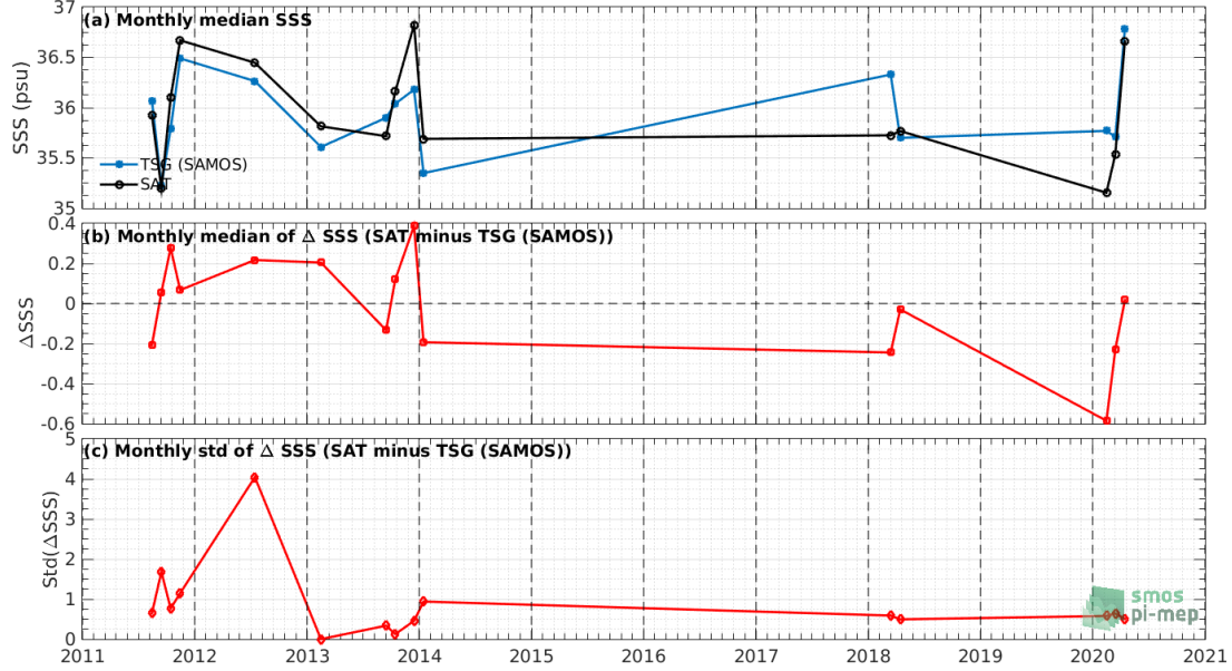
Figure 7: Time series of the monthly median SSS (top), median of \Delta\text{SSS} (Satellite - TSG (SAMOS)) and Std of \Delta\text{SSS} (Satellite - TSG (SAMOS)) over the South Atlantic Ocean Pi-MEP region considering all match-ups collected by the Pi-MEP.
