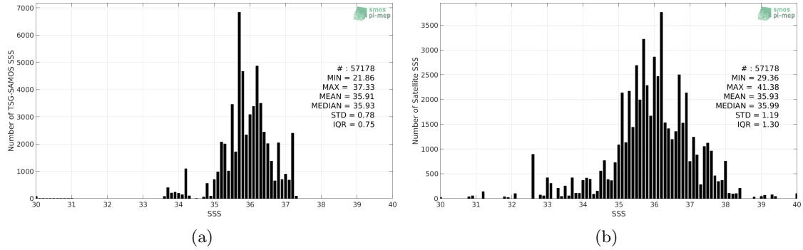
Figure 2: Histograms of SSS from TSG-SAMOS (a) and SMOS L2 v662 (ESA) (b) considering all match-up pairs per bins of 0.1 over the South Atlantic Ocean Pi-MEP region and for the full satellite product period.
