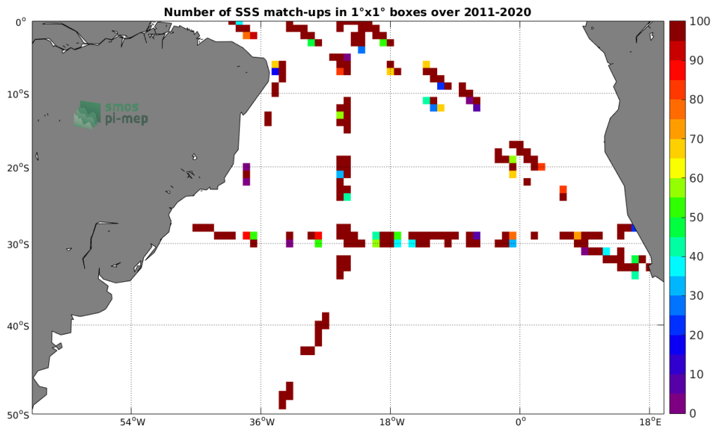
Figure 4: Number of SSS match-ups between TSG-SAMOS SSS and the SMOS L2 v662 (ESA) SSS product for the South Atlantic Ocean Pi-MEP region over 1^\circ \times 1^\circ boxes and for the full satellite product period.
