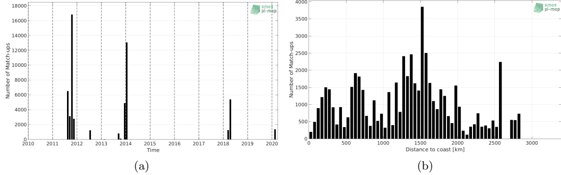
Figure 1: Number of match-ups between TSG-SAMOS and SMOS L2 v662 (ESA) SSS as a function of time (a) and as function of the distance to coast (b) over the South Atlantic Ocean Pi-MEP region and for the full satellite product period.
