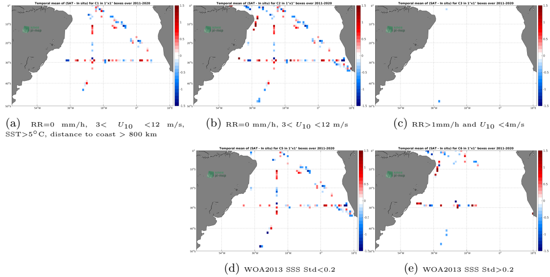
Figure 12: Temporal mean gridded over spatial boxes of size 1^\circ \times 1^\circ of \Delta SSS (SMOS L2 v662 (ESA) - TSG-SAMOS) for 5 different subdatasets corresponding to: RR=0 mm/h, 3 < U_{10} < 12 m/s, SST > 5^\circ C , distance to coast > 800 km (a), RR=0 mm/h, 3 < U_{10} < 12 m/s (b), RR > 1 mm/h and U_{10} < 4 m/s (c), WOA2013 SSS Std < 0.2 (d), WOA2013 SSS Std > 0.2 (e).
