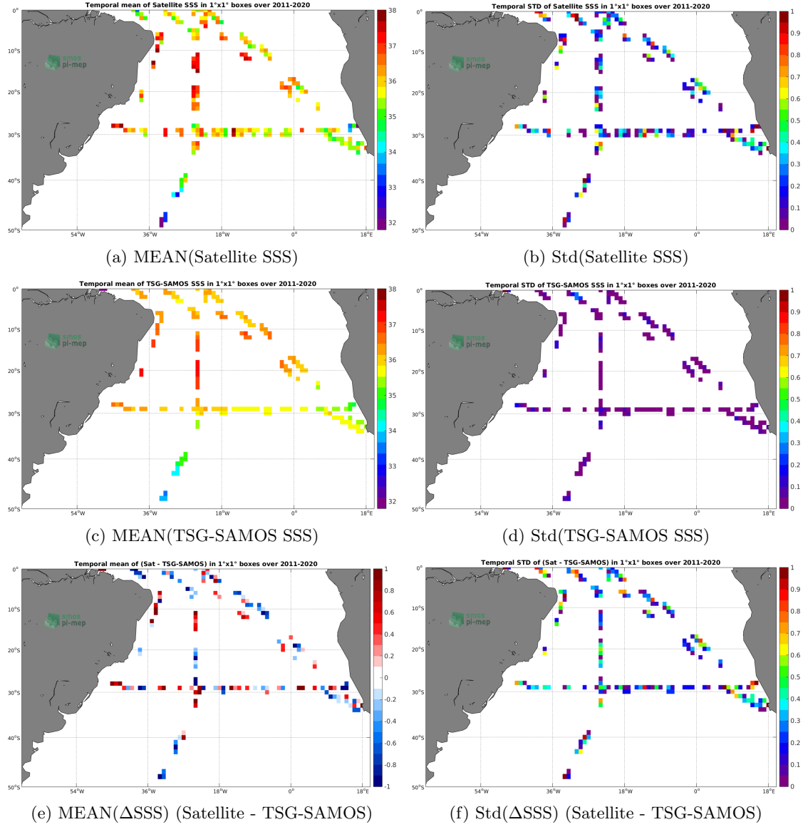
Figure 6: Temporal mean (left) and Std (right) of SSS from SMOS L2 v662 (ESA) (top), TSG-SAMOS (middle), and of \Delta SSS (Satellite - TSG-SAMOS). Only match-up pairs are used to generate these maps.
