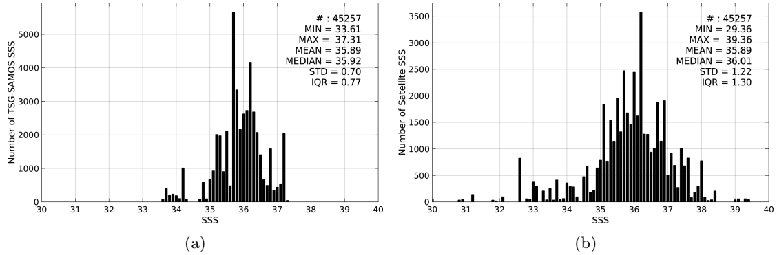
Figure 2: Histograms of SSS from TSG-SAMOS (a) and SMOS-L2-DPGS-v662 (b) considering all match-up pairs per bins of 0.1 over the South Atlantic Ocean Pi-MEP region and for the full satellite product period.
