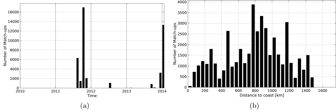
Figure 1: Number of match-ups between TSG-SAMOS and SMOS-L2-DPGS-v662 SSS as a function of time (a) and as function of the distance to coast (b) over the South Atlantic Ocean Pi-MEP region and for the full satellite product period.
