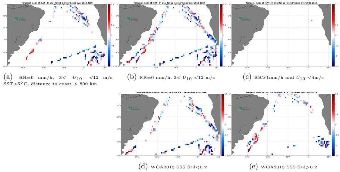
Figure 12: Temporal mean gridded over spatial boxes of size 1^\circ \times 1^\circ of \Delta SSS (SMOS SSS L2 v662 (ESA) - TSG (Polarstern)) for 5 different subdatasets corresponding to: RR=0 mm/h, 3 < U_{10} < 12 m/s, SST > 5^\circ C , distance to coast > 800 km (a), RR=0 mm/h, 3 < U_{10} < 12 m/s (b), RR > 1 mm/h and U_{10} < 4 m/s (c), WOA2013 SSS Std < 0.2 (d), WOA2013 SSS Std > 0.2 (e).
