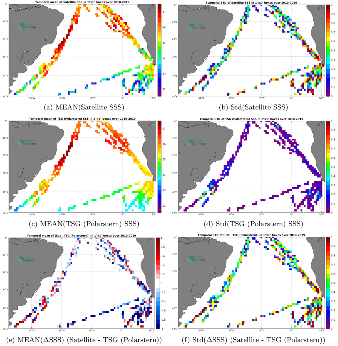
Figure 6: Temporal mean (left) and Std (right) of SSS from SMOS SSS L2 v662 (ESA) (top), TSG (Polarstern) (middle), and of \Delta SSS (Satellite - TSG (Polarstern)). Only match-up pairs are used to generate these maps.
