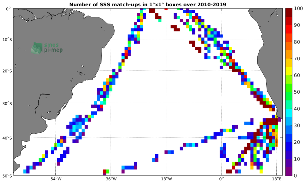
Figure 4: Number of SSS match-ups between TSG (Polarstern) SSS and the SMOS SSS L2 v662 (ESA) SSS product for the South Atlantic Ocean Pi-MEP region over 1^\circ \times 1^\circ boxes and for the full satellite product period.
