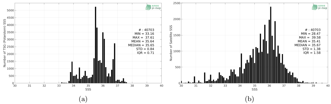
Figure 2: Histograms of SSS from TSG (Polarstern) (a) and SMOS SSS L2 v662 (ESA) (b) considering all match-up pairs per bins of 0.1 over the South Atlantic Ocean Pi-MEP region and for the full satellite product period.
