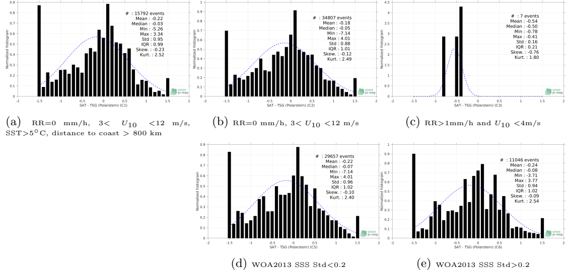
Figure 13: Normalized histogram of \Delta SSS (SMOS SSS L2 v662 (ESA) - TSG (Polarstern)) for 5 different subdatasets corresponding to: RR=0 mm/h, 3 < U_{10} < 12 m/s, SST>5°C, distance to coast > 800 km (a), RR=0 mm/h, 3 < U_{10} < 12 m/s (b), RR>1mm/h and U_{10} < 4 m/s (c), WOA2013 SSS Std<0.2 (d), WOA2013 SSS Std>0.2 (e).
