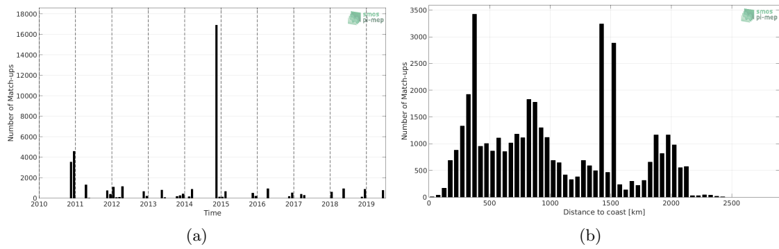
Figure 1: Number of match-ups between TSG (Polarstern) and SMOS SSS L2 v662 (ESA) SSS as a function of time (a) and as function of the distance to coast (b) over the South Atlantic Ocean Pi-MEP region and for the full satellite product period.
