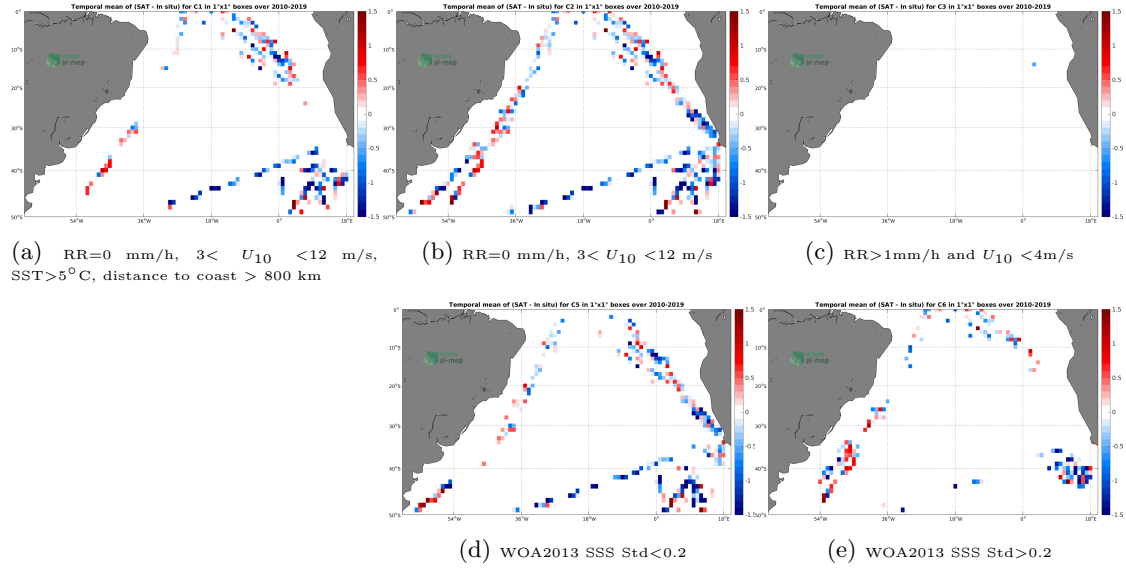
Figure 12: Temporal mean gridded over spatial boxes of size 1^\circ \times 1^\circ of \Delta SSS (SMOS L2 v662 (ESA) - TSG-POLARSTERN) for 5 different subdatasets corresponding to: RR=0 mm/h, 3 < U_{10} < 12 m/s, SST > 5^\circ C , distance to coast > 800 km (a), RR=0 mm/h, 3 < U_{10} < 12 m/s (b), RR > 1 mm/h and U_{10} < 4 m/s (c), WOA2013 SSS Std < 0.2 (d), WOA2013 SSS Std > 0.2 (e).
