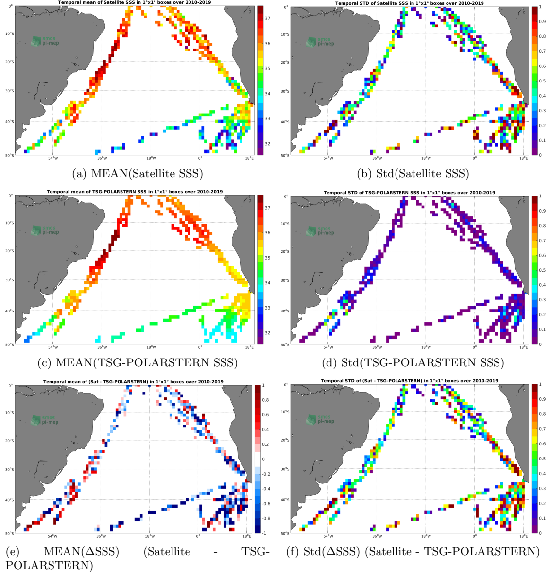
Figure 6: Temporal mean (left) and Std (right) of SSS from SMOS L2 v662 (ESA) (top), TSG-POLARSTERN (middle), and of \Delta SSS (Satellite - TSG-POLARSTERN). Only match-up pairs are used to generate these maps.
