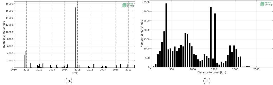
Figure 1: Number of match-ups between TSG-POLARSTERN and SMOS L2 v662 (ESA) SSS as a function of time (a) and as function of the distance to coast (b) over the South Atlantic Ocean Pi-MEP region and for the full satellite product period.
