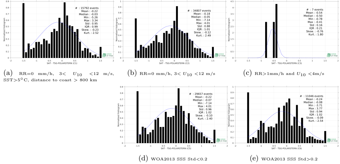
Figure 13: Normalized histogram of \Delta SSS (SMOS L2 v662 (ESA) - TSG-POLARSTERN) for 5 different subdatasets corresponding to: RR=0 mm/h, 3 < U_{10} < 12 m/s, SST > 5°C, distance to coast > 800 km (a), RR=0 mm/h, 3 < U_{10} < 12 m/s (b), RR > 1mm/h and U_{10} < 4 m/s (c), WOA2013 SSS Std < 0.2 (d), WOA2013 SSS Std > 0.2 (e).
