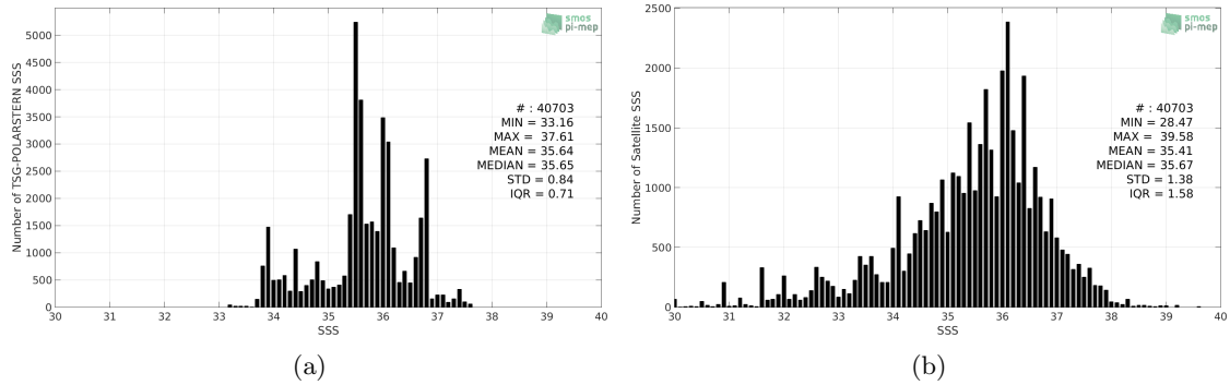
Figure 2: Histograms of SSS from TSG-POLARSTERN (a) and SMOS L2 v662 (ESA) (b) considering all match-up pairs per bins of 0.1 over the South Atlantic Ocean Pi-MEP region and for the full satellite product period.
