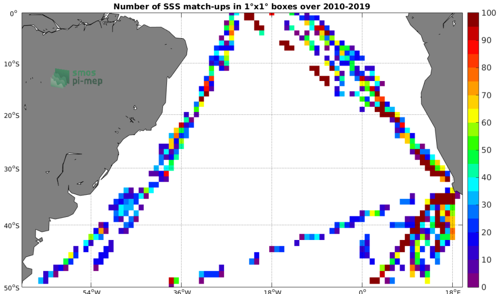
Figure 4: Number of SSS match-ups between TSG-POLARSTERN SSS and the SMOS L2 v662 (ESA) SSS product for the South Atlantic Ocean Pi-MEP region over 1°x1° boxes and for the full satellite product period.
