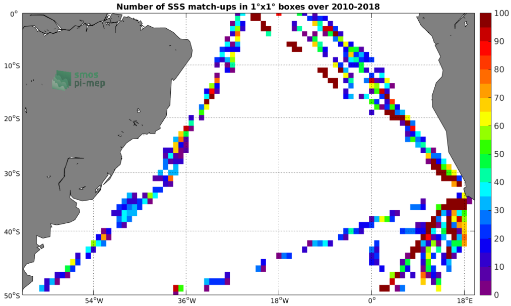
Figure 4: Number of SSS match-ups between TSG-POLARSTERN SSS and the SMOS-L2-DPGS-v662 SSS product for the South Atlantic Ocean Pi-MEP region over 1^\circ \times 1^\circ boxes and for the full satellite product period.
