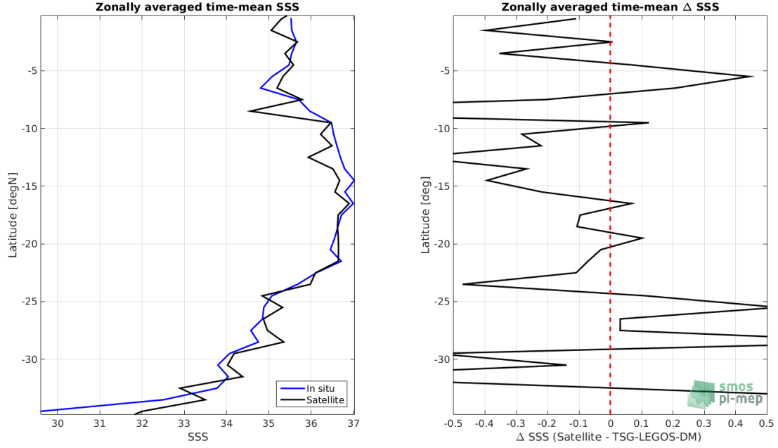
Figure 8: Left panel: Zonal mean SSS from SMOS L2 v662 (ESA) satellite product (black) and from TSG-LEGOS-DM (blue). Right panel: Zonal mean of \Delta SSS (Satellite - TSG-LEGOS-DM) for all the collected Pi-MEP match-up pairs estimated over the full satellite product period.
