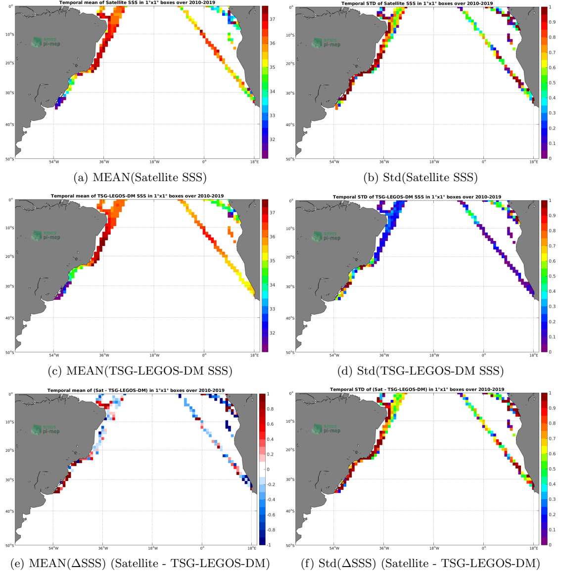
Figure 6: Temporal mean (left) and Std (right) of SSS from SMOS L2 v662 (ESA) (top), TSG-LEGOS-DM (middle), and of \Delta SSS (Satellite - TSG-LEGOS-DM). Only match-up pairs are used to generate these maps.
