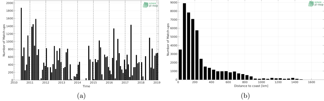
Figure 1: Number of match-ups between TSG-LEGOS-DM and SMOS L2 v662 (ESA) SSS as a function of time (a) and as function of the distance to coast (b) over the South Atlantic Ocean Pi-MEP region and for the full satellite product period.
