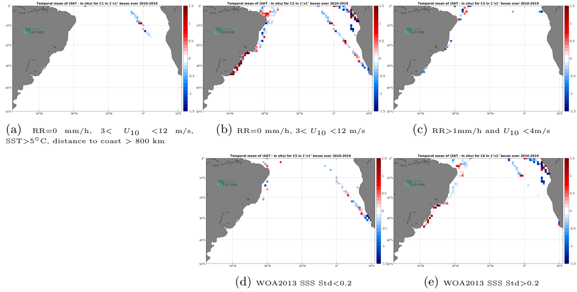
Figure 12: Temporal mean gridded over spatial boxes of size 1^\circ \times 1^\circ of \Delta SSS (SMOS L2 v662 (ESA) - TSG-LEGOS-DM) for 5 different subdatasets corresponding to: RR=0 mm/h, 3 < U_{10} < 12 m/s, SST > 5^\circ C , distance to coast > 800 km (a), RR=0 mm/h, 3 < U_{10} < 12 m/s (b), RR > 1 mm/h and U_{10} < 4 m/s (c), WOA2013 SSS Std < 0.2 (d), WOA2013 SSS Std > 0.2 (e).
