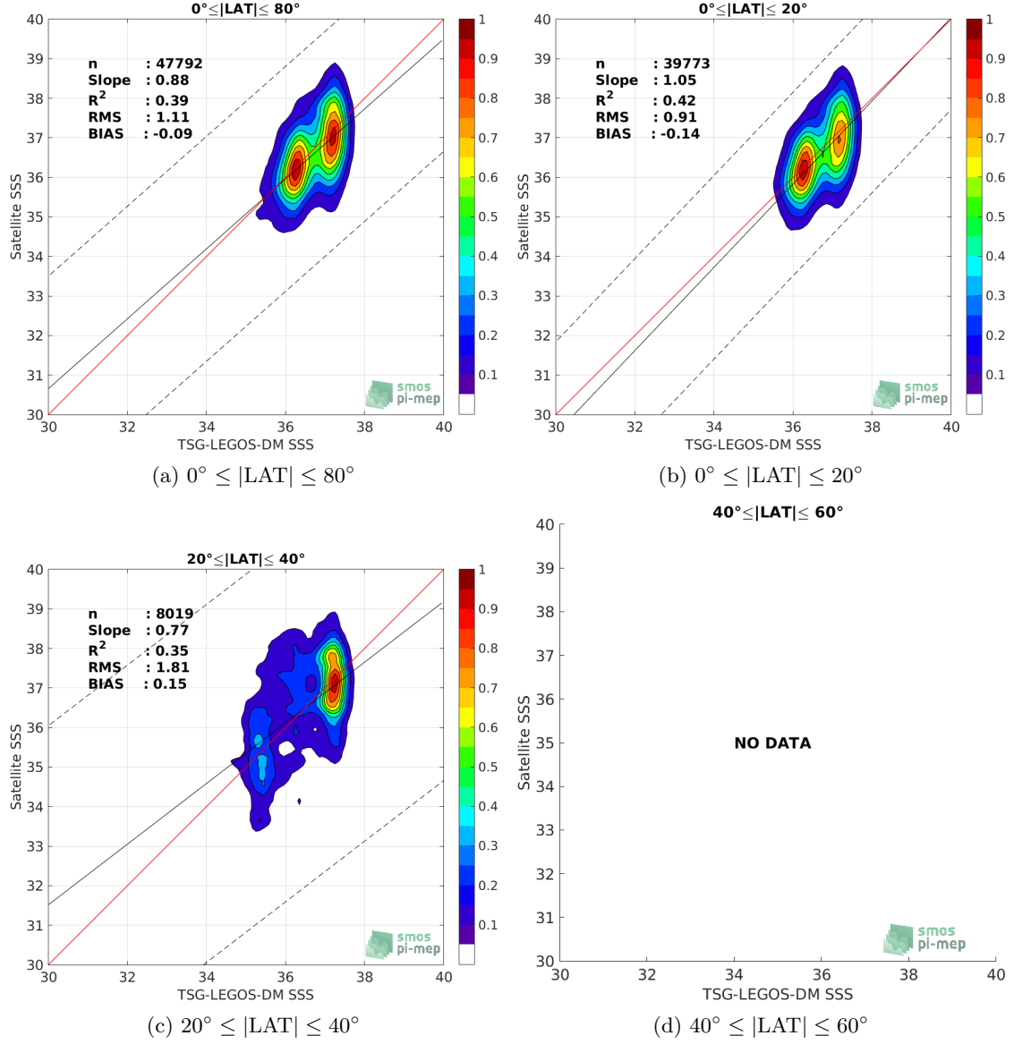
Figure 9: Contour maps of the concentration of SMOS L2 v662 (ESA) SSS (y-axis) versus TSG-LEGOS-DM SSS (x-axis) at match-up pairs for different latitude bands. For each plot, the red line shows x=y . The black thin and dashed lines indicate a linear fit through the data cloud and the \pm 95\% confidence levels, respectively. The number match-up pairs n , the slope and R^2 coefficient of the linear fit, the root mean square (RMS) and the mean bias between satellite and in situ data are indicated for each latitude band in each plots.
