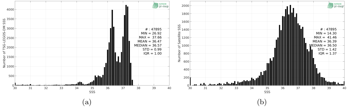
Figure 2: Histograms of SSS from TSG-LEGOS-DM (a) and SMOS L2 v662 (ESA) (b) considering all match-up pairs per bins of 0.1 over the South Atlantic Ocean Pi-MEP region and for the full satellite product period.
