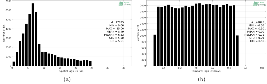
Figure 5: Histograms of the spatial (a) and temporal (b) lags between the time of the TSG-LEGOS-DM measurements and the date of the corresponding SMOS L2 v662 (ESA) SSS product.
