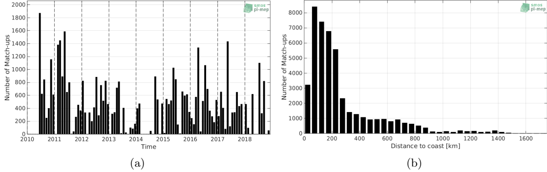
Figure 1: Number of match-ups between TSG-LEGOS-DM and SMOS-L2-DPGS-v662 SSS as a function of time (a) and as function of the distance to coast (b) over the South Atlantic Ocean Pi-MEP region and for the full satellite product period.
