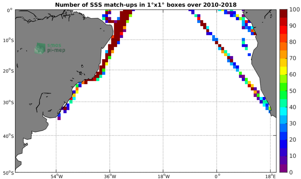
Figure 4: Number of SSS match-ups between TSG-LEGOS-DM SSS and the SMOS-L2-DPGS-v662 SSS product for the South Atlantic Ocean Pi-MEP region over 1^\circ \times 1^\circ boxes and for the full satellite product period.
