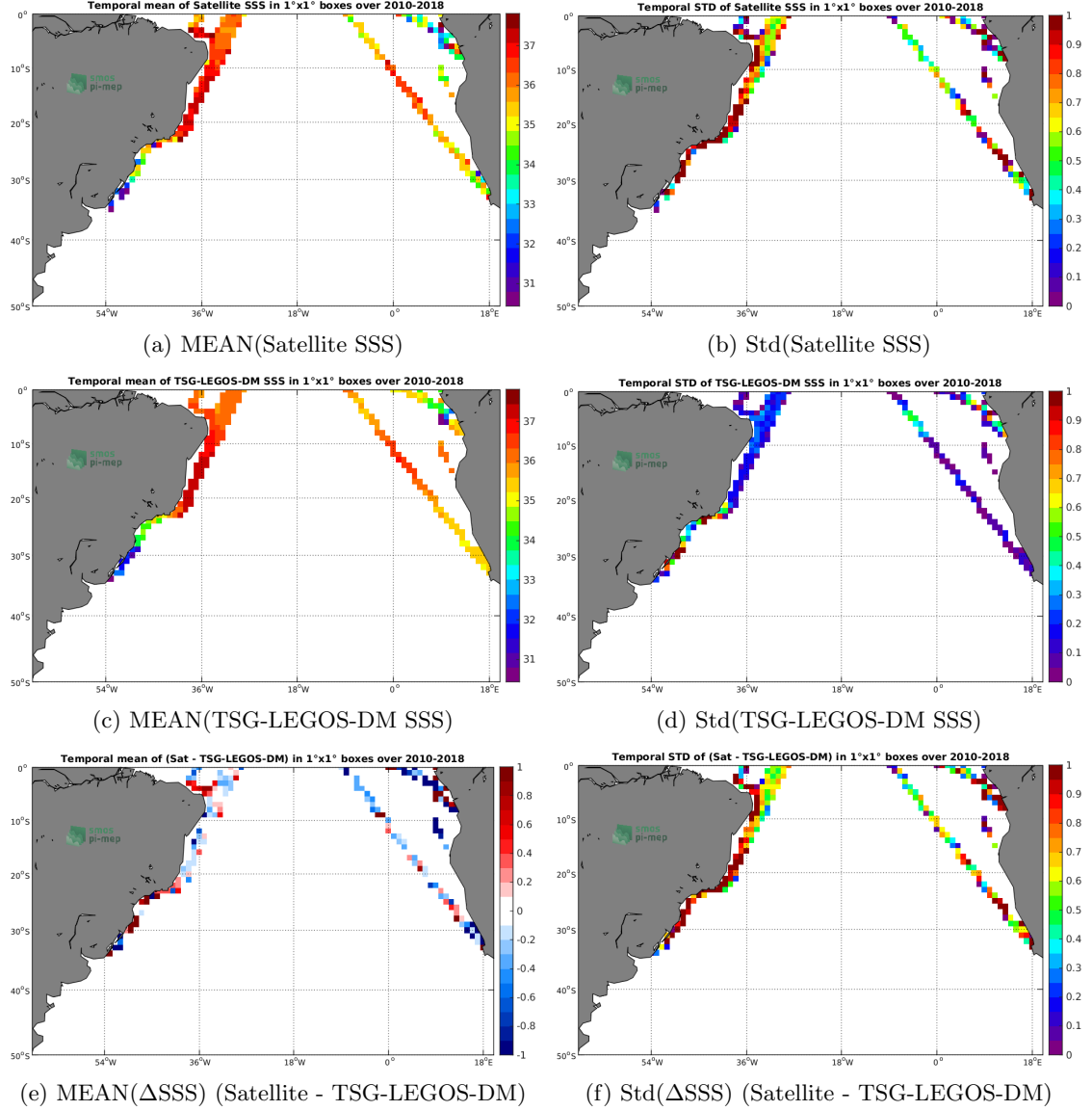
Figure 6: Temporal mean (left) and Std (right) of SSS from SMOS-L2-DPGS-v662 (top), TSG-LEGOS-DM (middle), and of \Delta SSS (Satellite - TSG-LEGOS-DM). Only match-up pairs are used to generate these maps.
