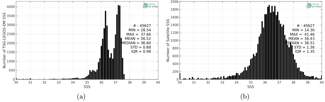
Figure 2: Histograms of SSS from TSG-LEGOS-DM (a) and SMOS-L2-DPGS-v662 (b) considering all match-up pairs per bins of 0.1 over the South Atlantic Ocean Pi-MEP region and for the full satellite product period.
