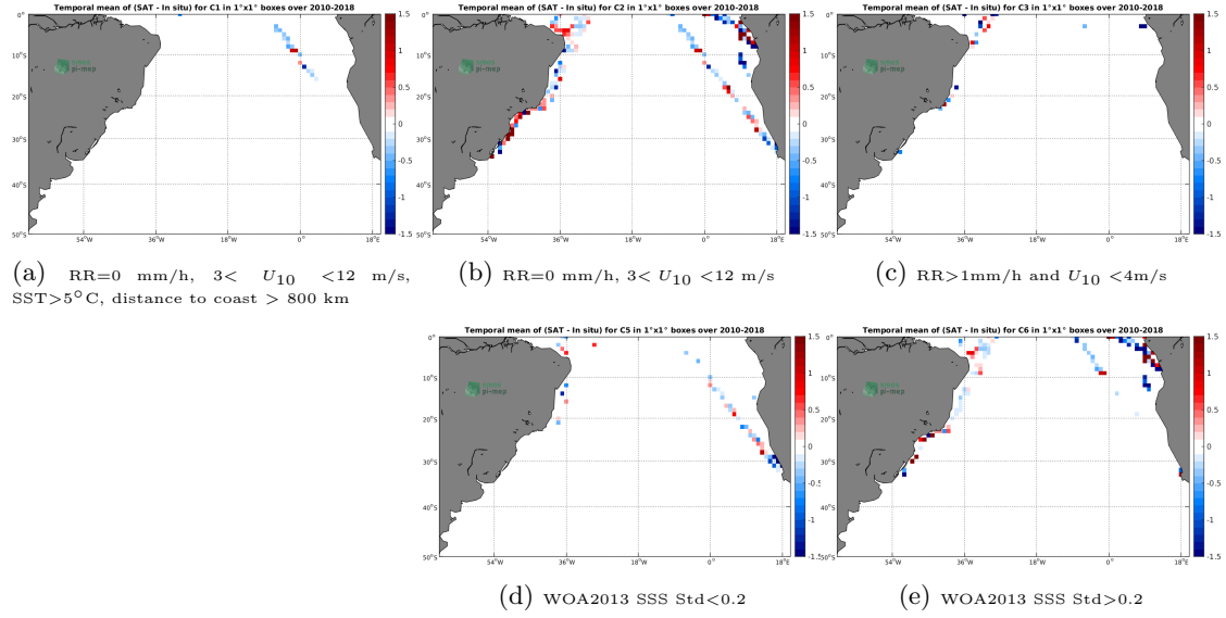
Figure 12: Temporal mean gridded over spatial boxes of size 1^\circ \times 1^\circ of \Delta SSS (SMOS-L2-DPGS-v662 - TSG-LEGOS-DM) for 5 different subdatasets corresponding to: RR=0 mm/h, 3 < U_{10} < 12 m/s, SST > 5^\circ C , distance to coast > 800 km (a), RR=0 mm/h, 3 < U_{10} < 12 m/s (b), RR > 1 mm/h and U_{10} < 4 m/s (c), WOA2013 SSS Std < 0.2 (d), WOA2013 SSS Std > 0.2 (e).
