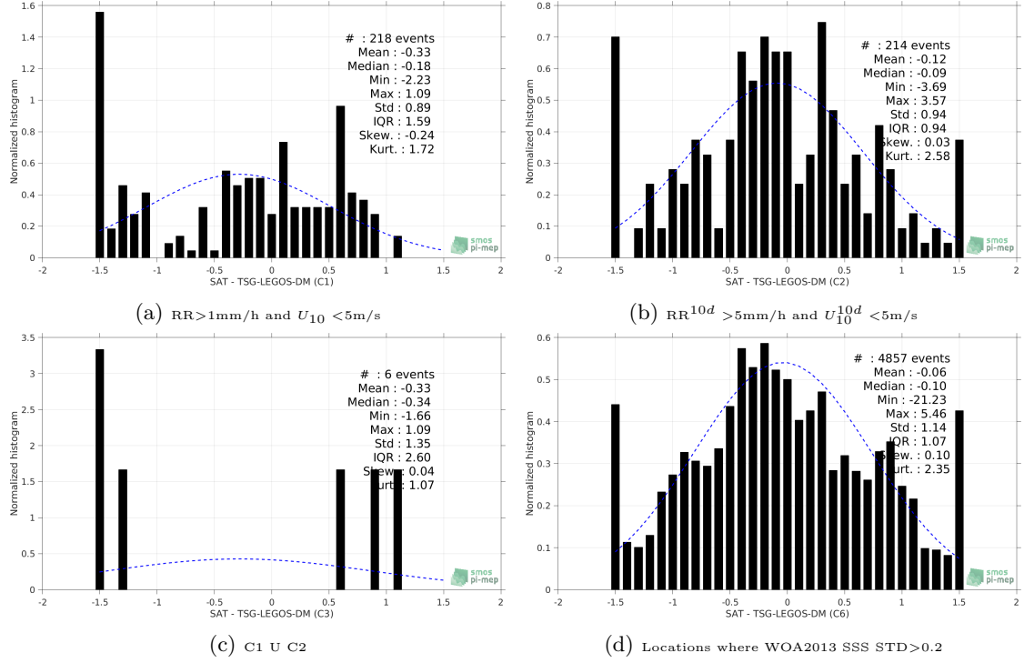
Figure 13: Normalized histogram of \Delta\text{SSS} (SMOS-L2-DPGS-v662 - TSG-LEGOS-DM) for 4 different subdatasets corresponding to: RR > 1mm/h and U_{10} < 5\text{m/s} (a), RR^{10d} > 5\text{mm/h} and U_{10}^{10d} < 5\text{m/s} (b), C1 U C2 (c), Locations where WOA2013 SSS STD > 0.2 (d).
