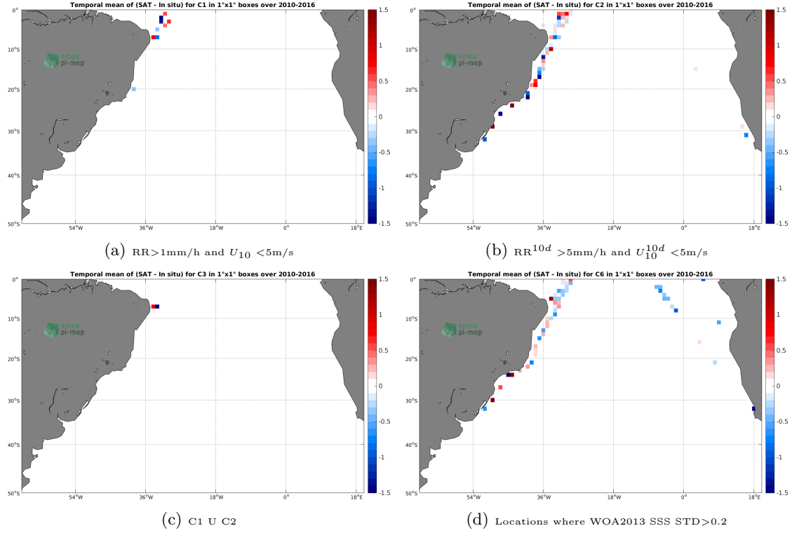
Figure 12: Temporal mean gridded over spatial boxes of size 1^\circ \times 1^\circ of \Delta SSS (SMOS-L2-DPGS-v662 - TSG-LEGOS-DM) for 4 different subdatasets corresponding to: RR > 1\text{mm/h} and U_{10} < 5\text{m/s} (a), RR^{10d} > 5\text{mm/h} and U_{10}^{10d} < 5\text{m/s} (b), C1 U C2 (c), Locations where WOA2013 SSS STD > 0.2 (d).
