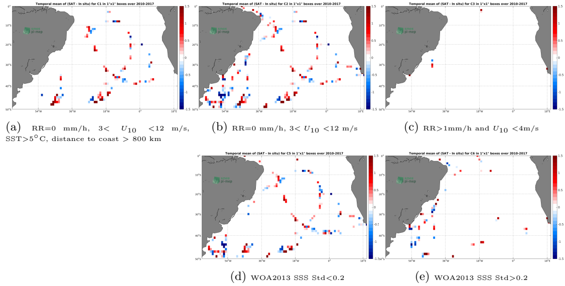
Figure 12: Temporal mean gridded over spatial boxes of size 1^\circ \times 1^\circ of \Delta SSS (SMOS L2 v662 (ESA) - TSG-GOSUD-Sailing-ship) for 5 different subdatasets corresponding to: RR=0 mm/h, 3 < U_{10} < 12 m/s, SST > 5^\circ C , distance to coast > 800 km (a), RR=0 mm/h, 3 < U_{10} < 12 m/s (b), RR > 1 mm/h and U_{10} < 4 m/s (c), WOA2013 SSS Std < 0.2 (d), WOA2013 SSS Std > 0.2 (e).
