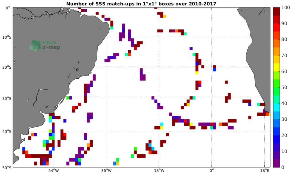
Figure 4: Number of SSS match-ups between TSG-GOSUD-Sailing-ship SSS and the SMOS L2 v662 (ESA) SSS product for the South Atlantic Ocean Pi-MEP region over 1^\circ \times 1^\circ boxes and for the full satellite product period.
