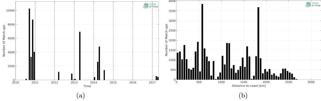
Figure 1: Number of match-ups between TSG-GOSUD-Sailing-ship and SMOS L2 v662 (ESA) SSS as a function of time (a) and as function of the distance to coast (b) over the South Atlantic Ocean Pi-MEP region and for the full satellite product period.
