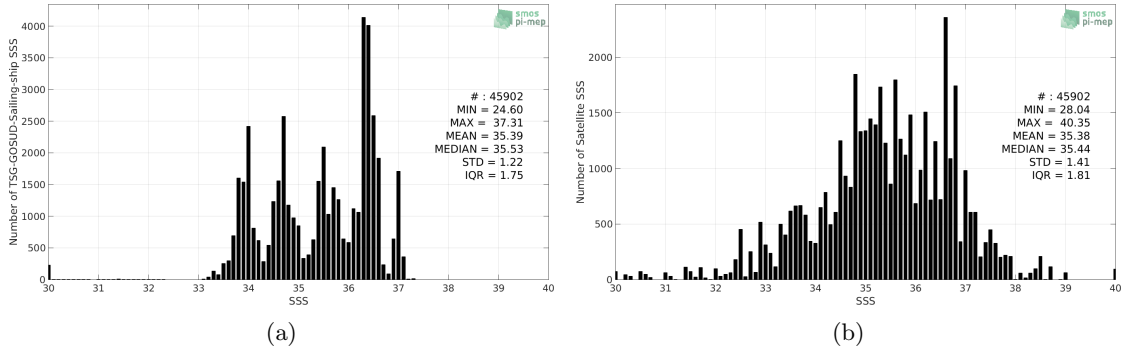
Figure 2: Histograms of SSS from TSG-GOSUD-Sailing-ship (a) and SMOS L2 v662 (ESA) (b) considering all match-up pairs per bins of 0.1 over the South Atlantic Ocean Pi-MEP region and for the full satellite product period.
