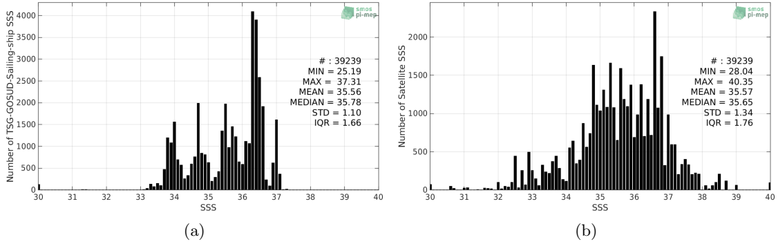
Figure 2: Histograms of SSS from TSG-GOSUD-Sailing-ship (a) and SMOS-L2-DPGS-v662 (b) considering all match-up pairs per bins of 0.1 over the South Atlantic Ocean Pi-MEP region and for the full satellite product period.
