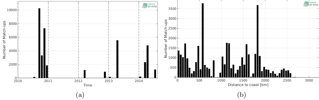
Figure 1: Number of match-ups between TSG-GOSUD-Sailing-ship and SMOS-L2-DPGS-v662 SSS as a function of time (a) and as function of the distance to coast (b) over the South Atlantic Ocean Pi-MEP region and for the full satellite product period.
