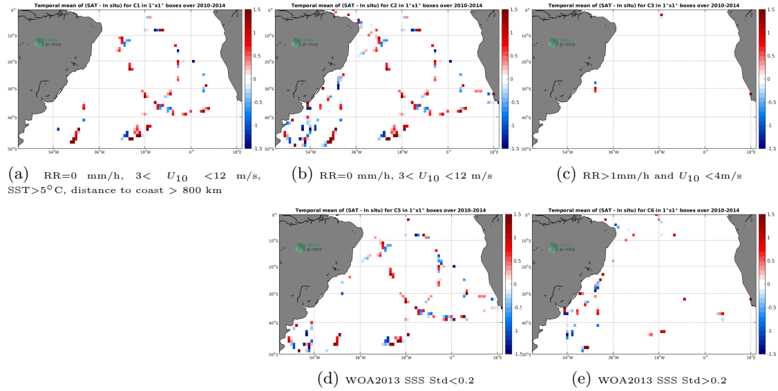
Figure 12: Temporal mean gridded over spatial boxes of size 1^\circ \times 1^\circ of \Delta SSS (SMOS-L2-DPGS-v662 - TSG-GOSUD-Sailing-ship) for 5 different subdatasets corresponding to:RR=0 mm/h, 3 < U_{10} < 12 m/s, SST >5^\circ\text{C} , distance to coast > 800 km (a), RR=0 mm/h, 3 < U_{10} < 12 m/s (b), RR >1 mm/h and U_{10} < 4 m/s (c), WOA2013 SSS Std <0.2 (d), WOA2013 SSS Std >0.2 (e).
