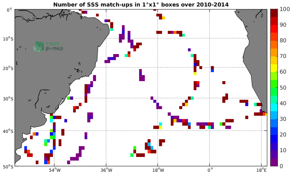
Figure 4: Number of SSS match-ups between TSG-GOSUD-Sailing-ship SSS and the SMOS-L2-DPGS-v662 SSS product for the South Atlantic Ocean Pi-MEP region over 1^\circ \times 1^\circ boxes and for the full satellite product period.
