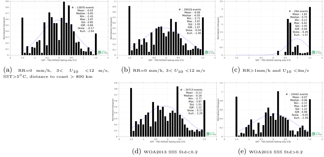
Figure 13: Normalized histogram of \Delta\text{SSS} (SMOS-L2-DPGS-v662 - TSG-GOSUD-Sailing-ship) for 5 different subdatasets corresponding to: RR=0 mm/h, 3 < U_{10} < 12 m/s, SST > 5^\circ\text{C} , distance to coast > 800 km (a), RR=0 mm/h, 3 < U_{10} < 12 m/s (b), RR > 1\text{mm/h} and U_{10} < 4\text{m/s} (c), WOA2013 SSS Std < 0.2 (d), WOA2013 SSS Std > 0.2 (e).
