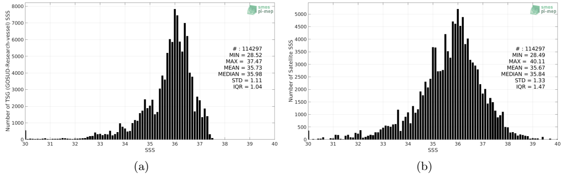
Figure 2: Histograms of SSS from TSG (GOSUD-Research-vessel) (a) and SMOS SSS L2 v662 (ESA) (b) considering all match-up pairs per bins of 0.1 over the South Atlantic Ocean Pi-MEP region and for the full satellite product period.
