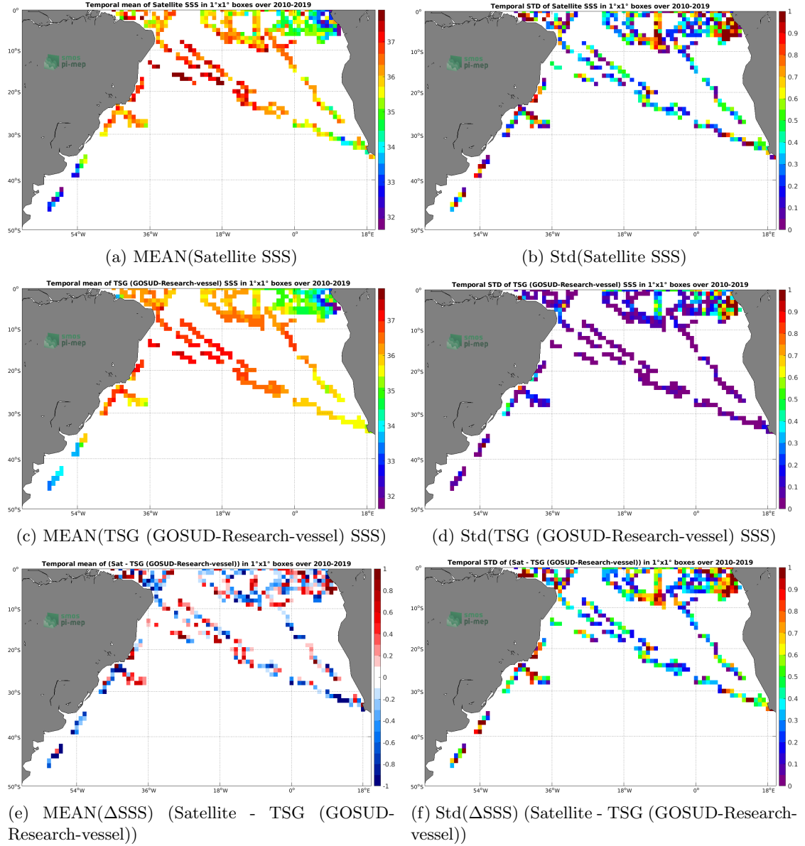
Figure 6: Temporal mean (left) and Std (right) of SSS from SMOS SSS L2 v662 (ESA) (top), TSG (GOSUD-Research-vessel) (middle), and of \Delta SSS (Satellite - TSG (GOSUD-Research-vessel)). Only match-up pairs are used to generate these maps.
