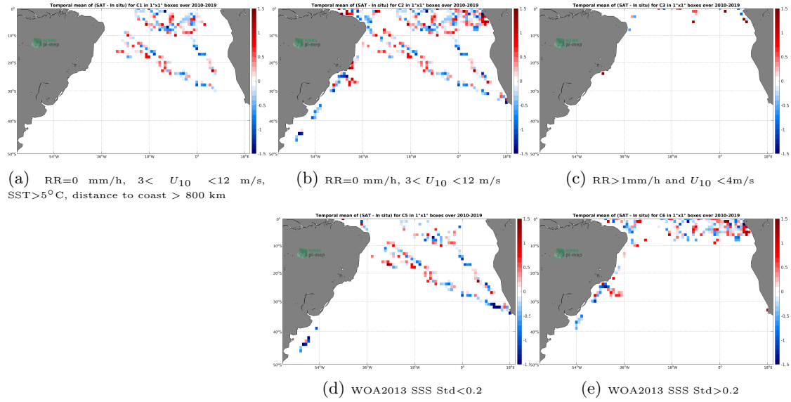
Figure 12: Temporal mean gridded over spatial boxes of size 1^\circ \times 1^\circ of \Delta SSS (SMOS SSS L2 v662 (ESA) - TSG (GOSUD-Research-vessel)) for 5 different subdatasets corresponding to: RR=0 mm/h, 3 < U_{10} < 12 m/s, SST > 5^\circ C , distance to coast > 800 km (a), RR=0 mm/h, 3 < U_{10} < 12 m/s (b), RR > 1 mm/h and U_{10} < 4 m/s (c), WOA2013 SSS Std < 0.2 (d), WOA2013 SSS Std > 0.2 (e).
