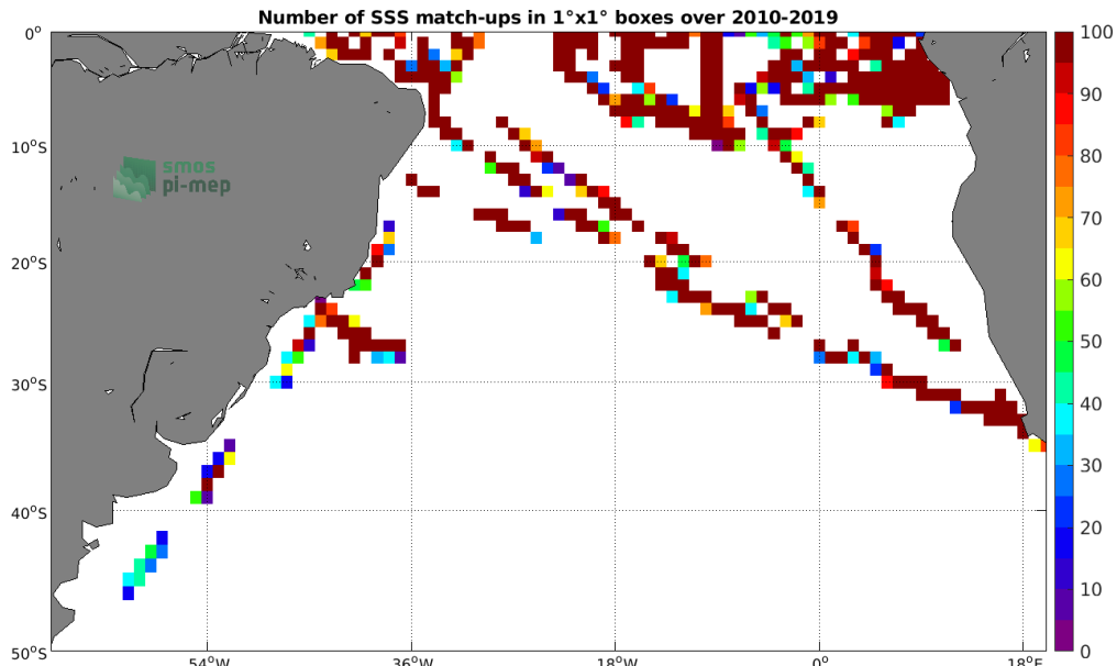
Figure 4: Number of SSS match-ups between TSG (GOSUD-Research-vessel) SSS and the SMOS SSS L2 v662 (ESA) SSS product for the South Atlantic Ocean Pi-MEP region over 1^\circ \times 1^\circ boxes and for the full satellite product period.
