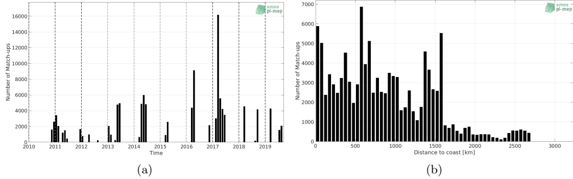
Figure 1: Number of match-ups between TSG (GOSUD-Research-vessel) and SMOS SSS L2 v662 (ESA) SSS as a function of time (a) and as function of the distance to coast (b) over the South Atlantic Ocean Pi-MEP region and for the full satellite product period.
