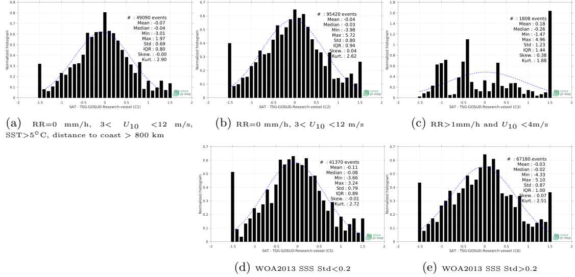
Figure 13: Normalized histogram of \Delta SSS (SMOS L2 v662 (ESA) - TSG-GOSUD-Research-vessel) for 5 different subdatasets corresponding to: RR=0 mm/h, 3 < U_{10} < 12 m/s, SST > 5°C, distance to coast > 800 km (a), RR=0 mm/h, 3 < U_{10} < 12 m/s (b), RR > 1mm/h and U_{10} < 4 m/s (c), WOA2013 SSS Std < 0.2 (d), WOA2013 SSS Std > 0.2 (e).
