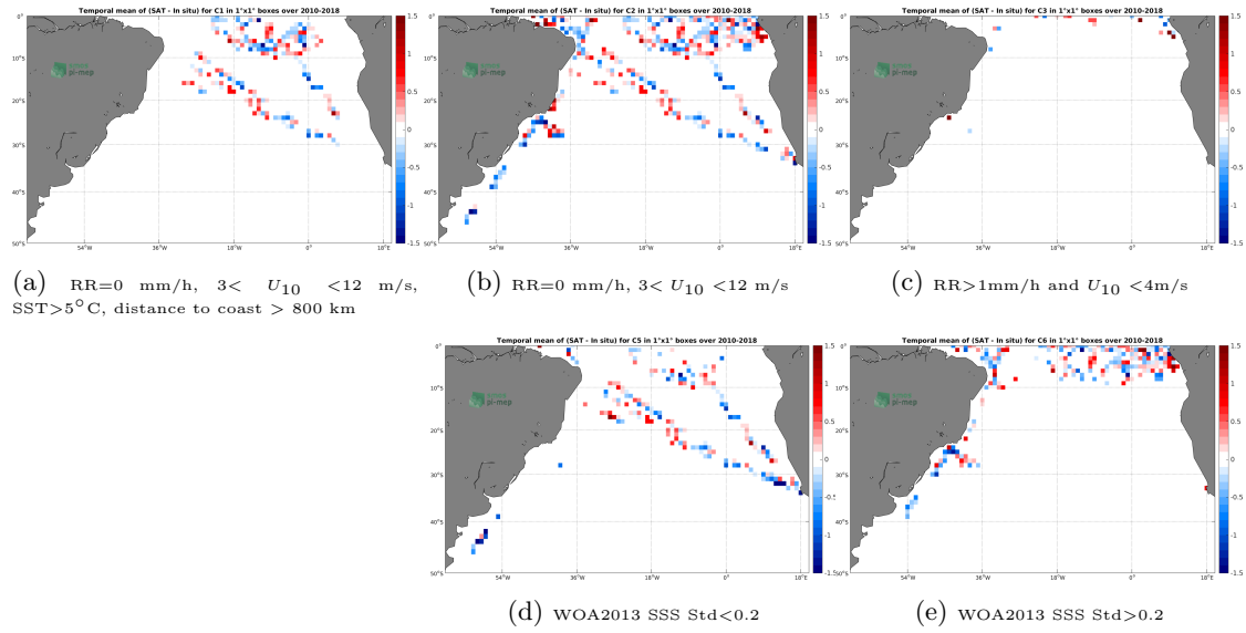
Figure 12: Temporal mean gridded over spatial boxes of size 1^\circ \times 1^\circ of \Delta SSS (SMOS L2 v662 (ESA) - TSG-GOSUD-Research-vessel) for 5 different subdatasets corresponding to: RR=0 mm/h, 3 < U_{10} < 12 m/s, SST > 5^\circ C , distance to coast > 800 km (a), RR=0 mm/h, 3 < U_{10} < 12 m/s (b), RR > 1 mm/h and U_{10} < 4 m/s (c), WOA2013 SSS Std < 0.2 (d), WOA2013 SSS Std > 0.2 (e).
