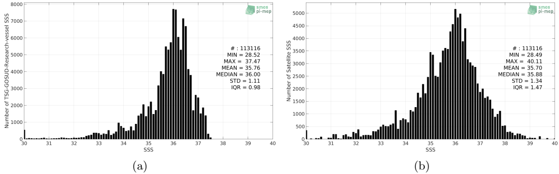
Figure 2: Histograms of SSS from TSG-GOSUD-Research-vessel (a) and SMOS L2 v662 (ESA) (b) considering all match-up pairs per bins of 0.1 over the South Atlantic Ocean Pi-MEP region and for the full satellite product period.
