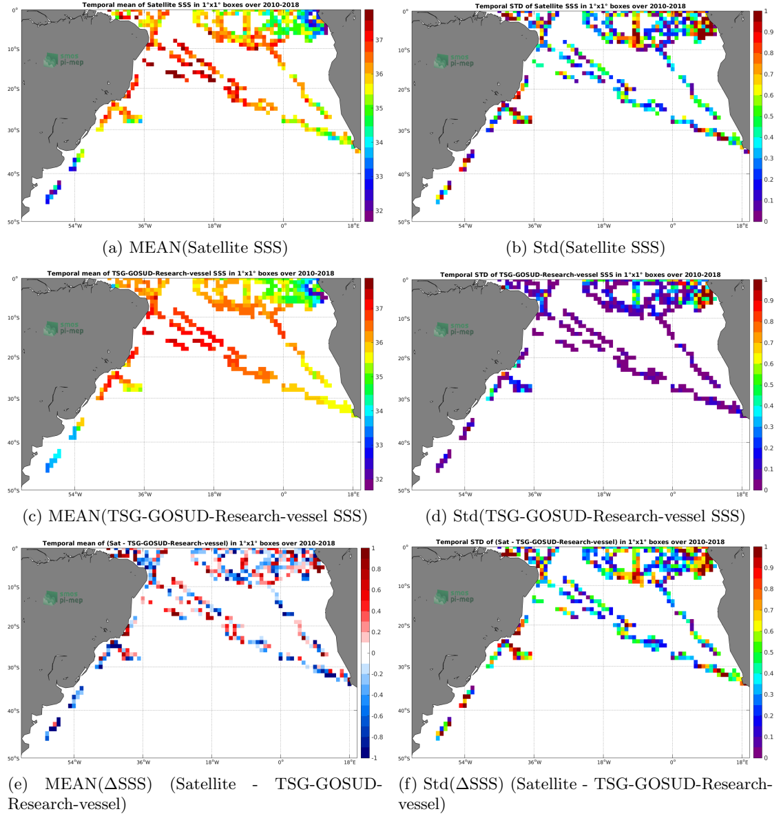
Figure 6: Temporal mean (left) and Std (right) of SSS from SMOS L2 v662 (ESA) (top), TSG-GOSUD-Research-vessel (middle), and of \Delta SSS (Satellite - TSG-GOSUD-Research-vessel). Only match-up pairs are used to generate these maps.
