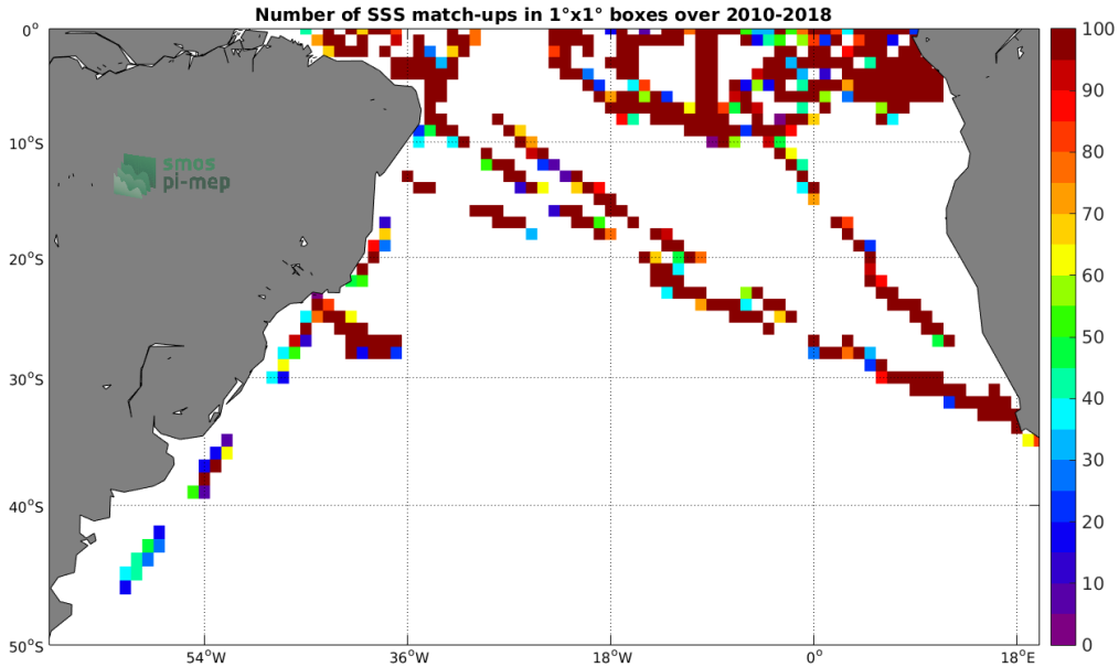
Figure 4: Number of SSS match-ups between TSG-GOSUD-Research-vessel SSS and the SMOS L2 v662 (ESA) SSS product for the South Atlantic Ocean Pi-MEP region over 1°x1° boxes and for the full satellite product period.
