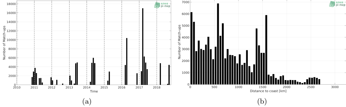
Figure 1: Number of match-ups between TSG-GOSUD-Research-vessel and SMOS L2 v662 (ESA) SSS as a function of time (a) and as function of the distance to coast (b) over the South Atlantic Ocean Pi-MEP region and for the full satellite product period.
