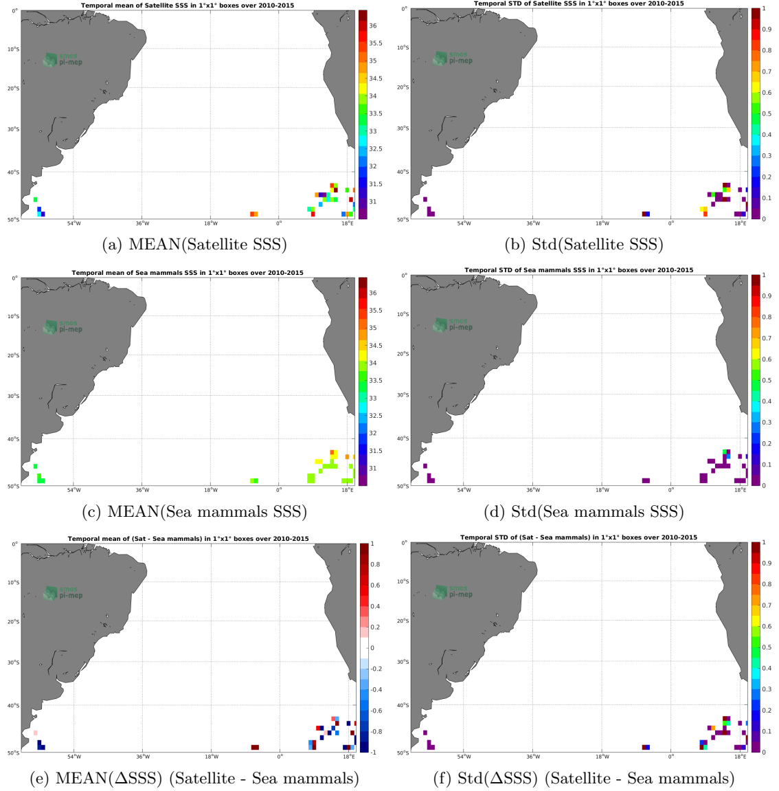
Figure 6: Temporal mean (left) and Std (right) of SSS from SMOS L2 v662 (ESA) (top), Sea mammals (middle), and of \Delta SSS (Satellite - Sea mammals). Only match-up pairs are used to generate these maps.
