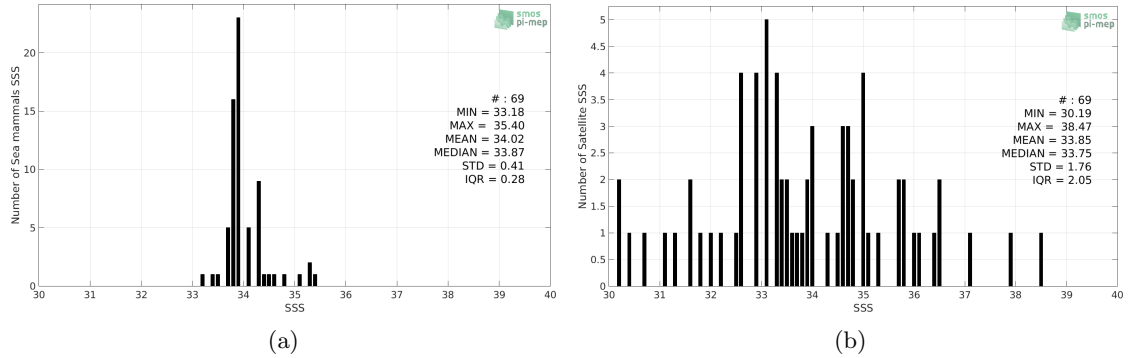
Figure 2: Histograms of SSS from Sea mammals (a) and SMOS L2 v662 (ESA) (b) considering all match-up pairs per bins of 0.1 over the South Atlantic Ocean Pi-MEP region and for the full satellite product period.
