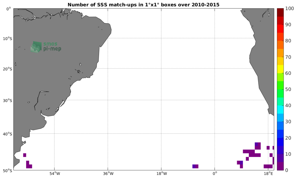
Figure 4: Number of SSS match-ups between Sea mammals SSS and the SMOS L2 v662 (ESA) SSS product for the South Atlantic Ocean Pi-MEP region over 1°x1° boxes and for the full satellite product period.
