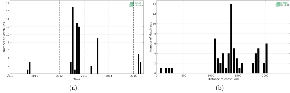
Figure 1: Number of match-ups between Sea mammals and SMOS L2 v662 (ESA) SSS as a function of time (a) and as function of the distance to coast (b) over the South Atlantic Ocean Pi-MEP region and for the full satellite product period.
