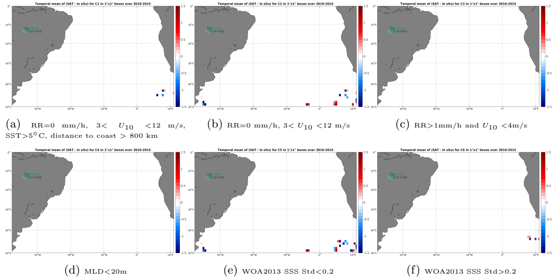
Figure 12: Temporal mean gridded over spatial boxes of size 1^{\circ}\times 1^{\circ} of \Delta\text{SSS} (SMOS L2 v662 (ESA) - Sea mammals) for 6 different subdatasets corresponding to: \text{RR}=0 mm/h, 3 < U_{10} < 12 m/s, SST > 5^{\circ}\text{C} , distance to coast > 800 km (a), \text{RR}=0 mm/h, 3 < U_{10} < 12 m/s (b), \text{RR} > 1\text{mm/h} and U_{10} < 4\text{m/s} (c), \text{MLD} < 20\text{m} (d), \text{WOA2013 SSS Std} < 0.2 (e), \text{WOA2013 SSS Std} > 0.2 (f).
