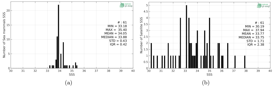
Figure 2: Histograms of SSS from Sea mammals (a) and SMOS-L2-DPGS-v662 (b) considering all match-up pairs per bins of 0.1 over the South Atlantic Ocean Pi-MEP region and for the full satellite product period.
