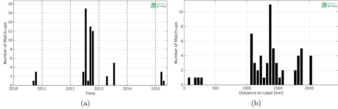
Figure 1: Number of match-ups between Sea mammals and SMOS-L2-DPGS-v662 SSS as a function of time (a) and as function of the distance to coast (b) over the South Atlantic Ocean Pi-MEP region and for the full satellite product period.
