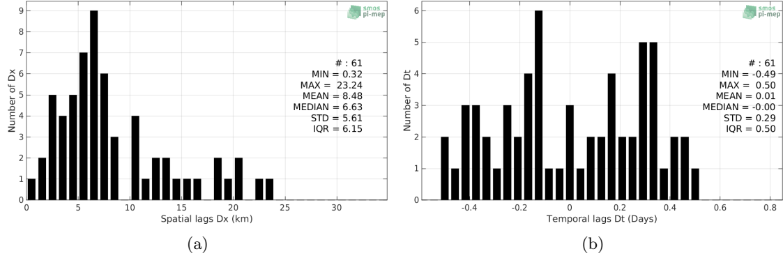
Figure 5: Histograms of the spatial (a) and temporal (b) lags between the time of the Sea mammals measurements and the date of the corresponding SMOS-L2-DPGS-v662 SSS product.
