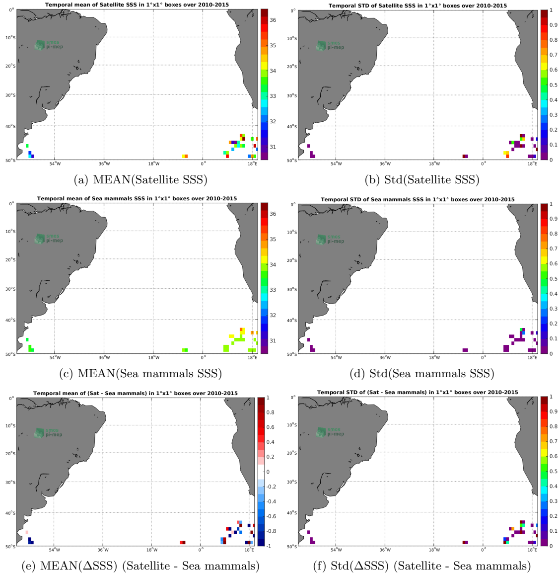
Figure 6: Temporal mean (left) and Std (right) of SSS from SMOS-L2-DPGS-v662 (top), Sea mammals (middle), and of \Delta SSS (Satellite - Sea mammals). Only match-up pairs are used to generate these maps.
