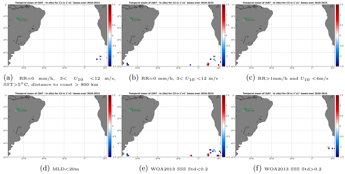
Figure 12: Temporal mean gridded over spatial boxes of size 1^\circ \times 1^\circ of \Delta SSS (SMOS-L2-DPGS-v662 - Sea mammals) for 6 different subdatasets corresponding to: RR=0 mm/h, 3 < U_{10} < 12 m/s, SST >5^\circ\text{C} , distance to coast > 800 km (a), RR=0 mm/h, 3 < U_{10} < 12 m/s (b), RR >1 mm/h and U_{10} < 4 m/s (c),MLD <20 m (d),WOA2013 SSS Std <0.2 (e),WOA2013 SSS Std >0.2 (f).
