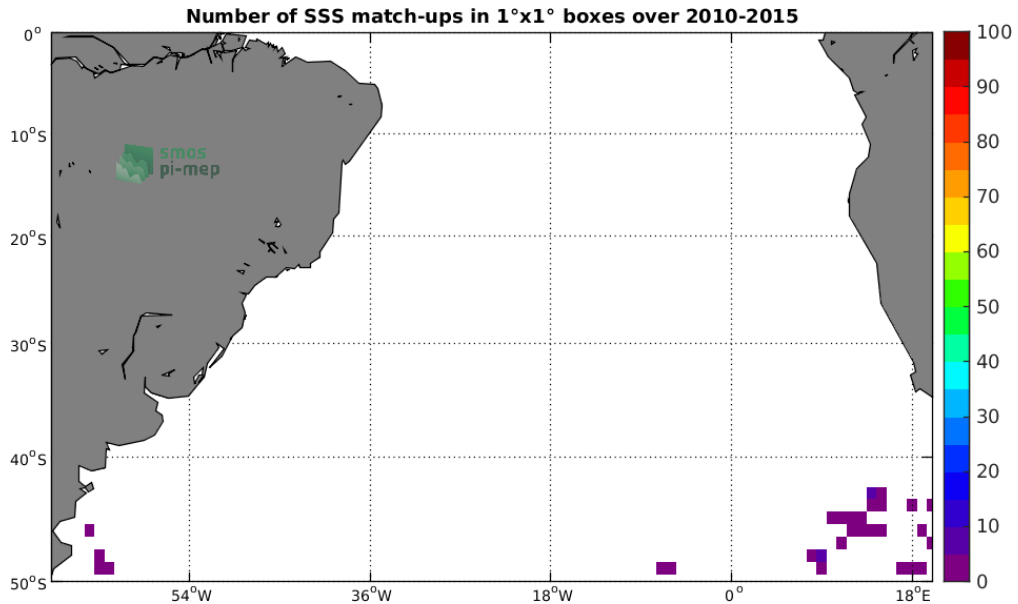
Figure 4: Number of SSS match-ups between Sea mammals SSS and the SMOS-L2-DPGS-v662 SSS product for the South Atlantic Ocean Pi-MEP region over 1°x1° boxes and for the full satellite product period.
