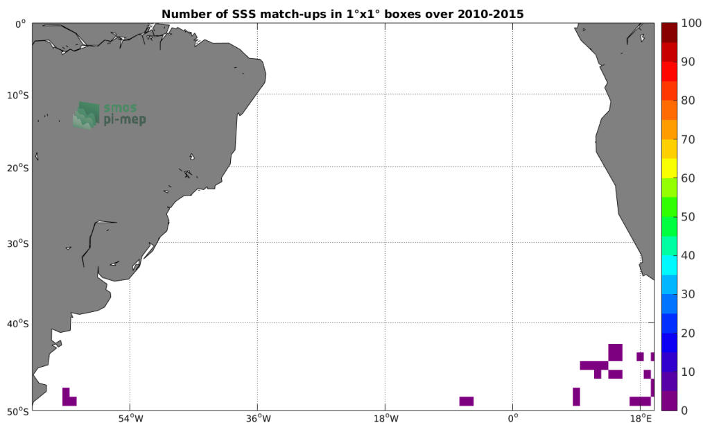
Figure 4: Number of SSS match-ups between Sea mammals SSS and the SMOS-L2-DPGS-v662 SSS product for the South Atlantic Ocean Pi-MEP region over 1^\circ \times 1^\circ boxes and for the full satellite product period.
