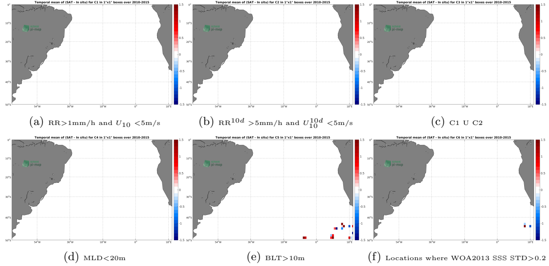
Figure 12: Temporal mean gridded over spatial boxes of size 1^\circ \times 1^\circ of \Delta\text{SSS} (SMOS-L2-DPGS-v662 - Sea mammals) for 6 different subdatasets corresponding to: RR > 1\text{mm/h} and U_{10} < 5\text{m/s} (a), RR^{10d} > 5\text{mm/h} and U_{10}^{10d} < 5\text{m/s} (b), C1 U C2 (c), MLD < 20\text{m} (d), BLT > 10\text{m} (e), Locations where WOA2013 SSS STD > 0.2 (f).
