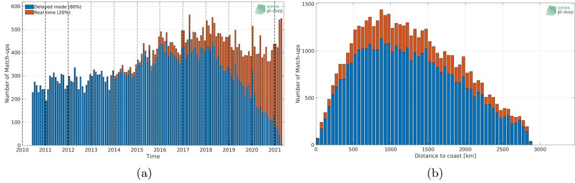
Figure 1: Number of match-ups between Argo and SMOS SSS L2 v662 (ESA) SSS as a function of time (a) and as function of the distance to coast (b) over the South Atlantic Ocean Pi-MEP region and for the full satellite product period.
