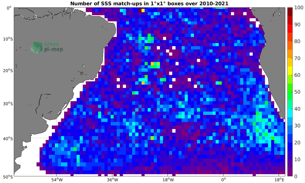
Figure 4: Number of SSS match-ups between Argo SSS and the SMOS SSS L2 v662 (ESA) SSS product for the South Atlantic Ocean Pi-MEP region over 1^\circ \times 1^\circ boxes and for the full satellite product period.
