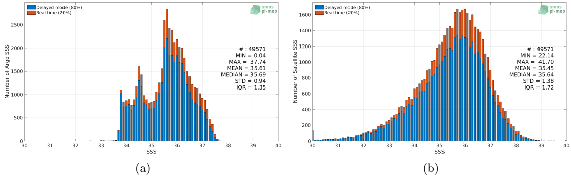
Figure 2: Histograms of SSS from Argo (a) and SMOS SSS L2 v662 (ESA) (b) considering all match-up pairs per bins of 0.1 over the South Atlantic Ocean Pi-MEP region and for the full satellite product period.
