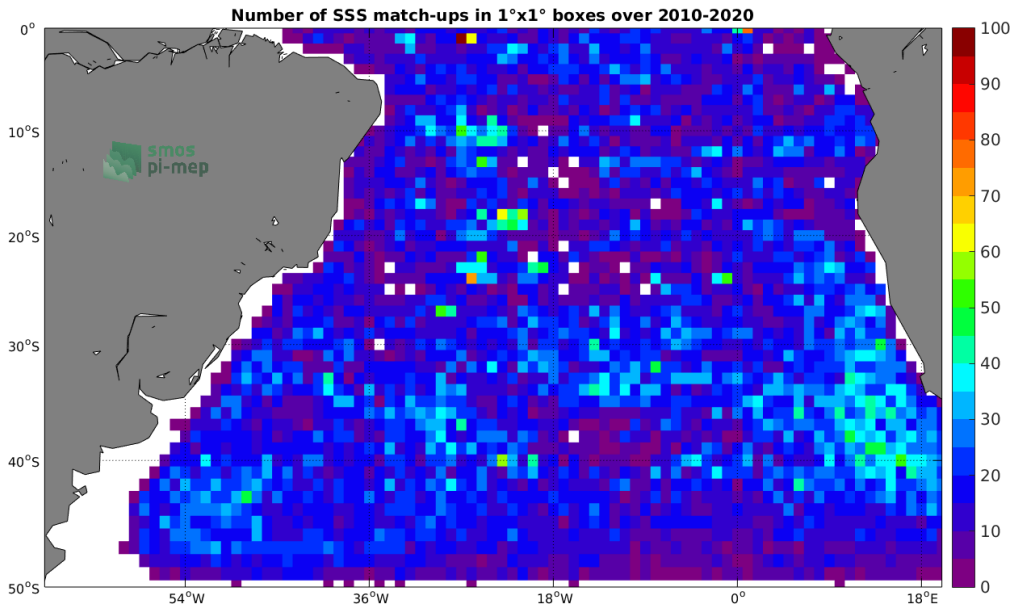
Figure 4: Number of SSS match-ups between Argo SSS and the SMOS SSS L2 v662 (ESA) SSS product for the South Atlantic Ocean Pi-MEP region over 1°x1° boxes and for the full satellite product period.
