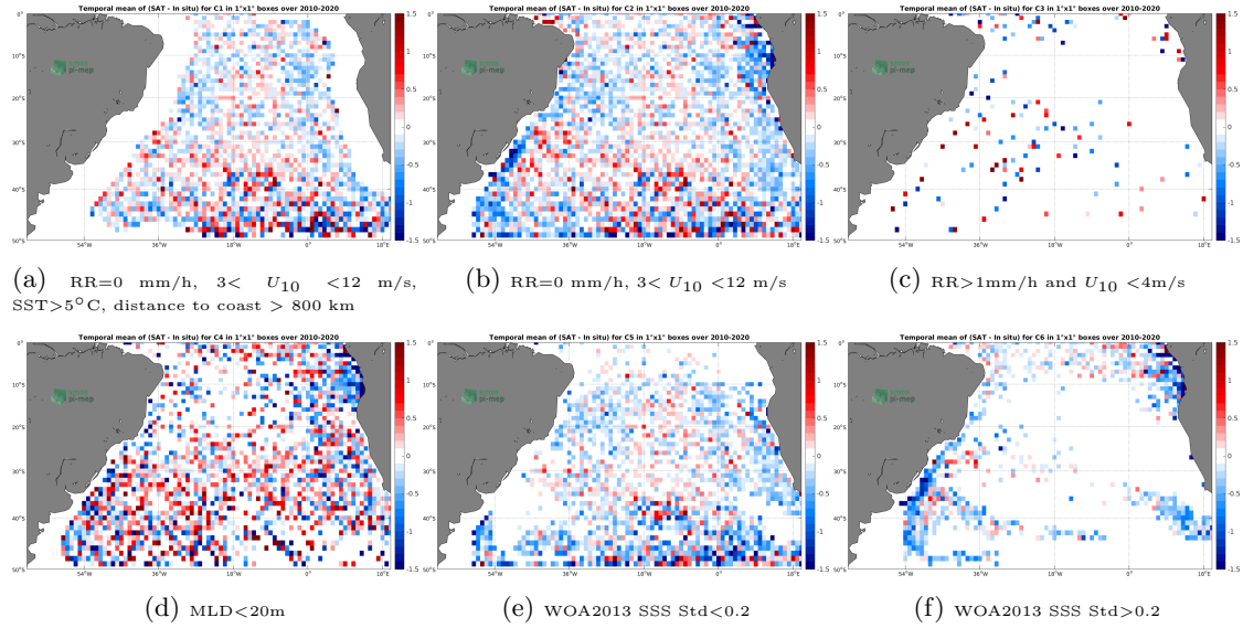
Figure 12: Temporal mean gridded over spatial boxes of size 1^\circ \times 1^\circ of \Delta SSS (SMOS SSS L2 v662 (ESA) - Argo) for 6 different subdatasets corresponding to: RR=0 mm/h, 3 < U_{10} < 12 m/s, SST > 5^\circ C , distance to coast > 800 km (a), RR=0 mm/h, 3 < U_{10} < 12 m/s (b), RR > 1 mm/h and U_{10} < 4 m/s (c), MLD < 20 m (d), WOA2013 SSS Std < 0.2 (e), WOA2013 SSS Std > 0.2 (f).
