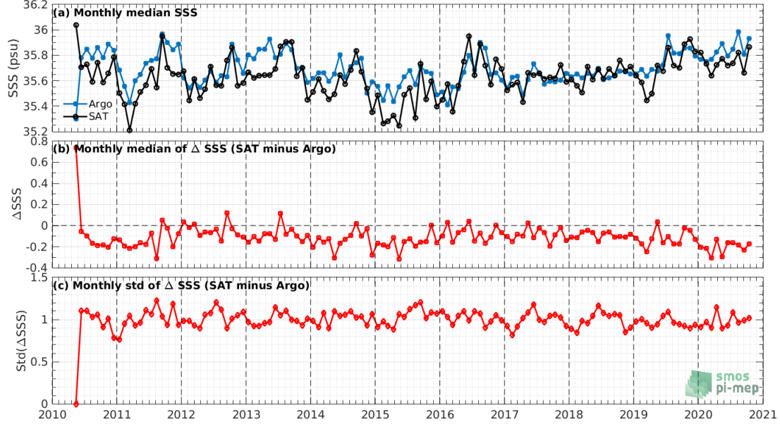
Figure 7: Time series of the monthly median SSS (top), median of \Delta\text{SSS} (Satellite - Argo) and Std of \Delta\text{SSS} (Satellite - Argo) over the South Atlantic Ocean Pi-MEP region considering all match-ups collected by the Pi-MEP.
