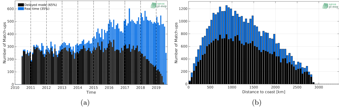
Figure 1: Number of match-ups between Argo and SMOS-L2-DPGS-v662 SSS as a function of time (a) and as function of the distance to coast (b) over the South Atlantic Ocean Pi-MEP region and for the full satellite product period.
