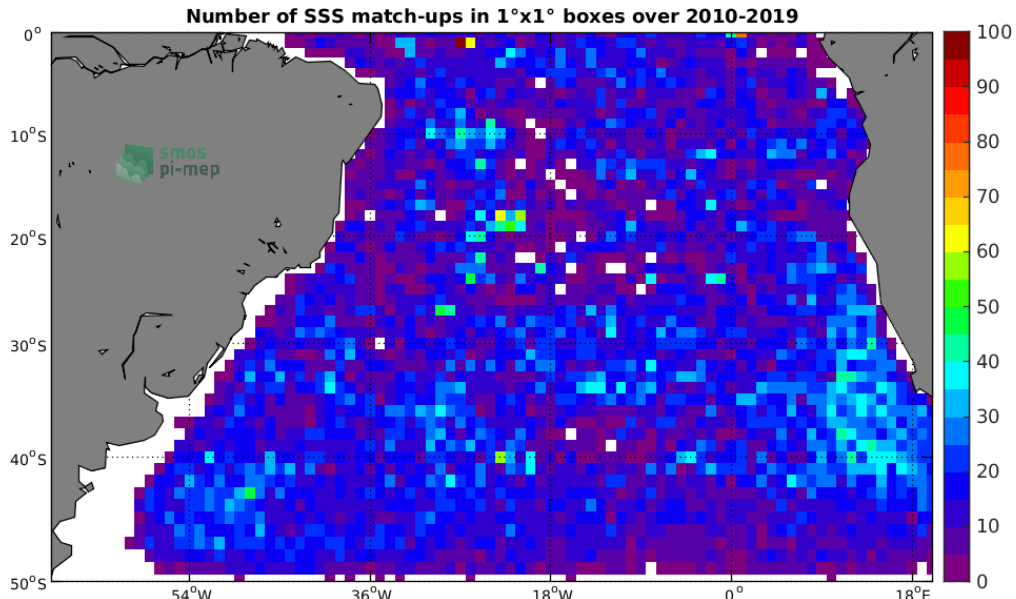
Figure 4: Number of SSS match-ups between Argo SSS and the SMOS-L2-DPGS-v662 SSS product for the South Atlantic Ocean Pi-MEP region over 1°x1° boxes and for the full satellite product period.
