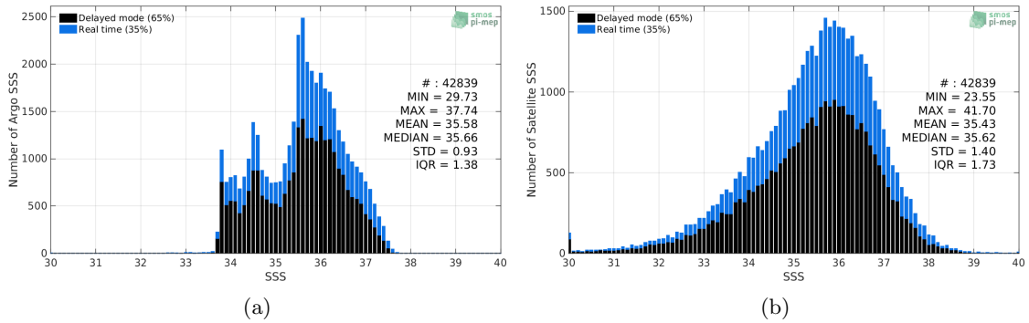
Figure 2: Histograms of SSS from Argo (a) and SMOS-L2-DPGS-v662 (b) considering all match-up pairs per bins of 0.1 over the South Atlantic Ocean Pi-MEP region and for the full satellite product period.
