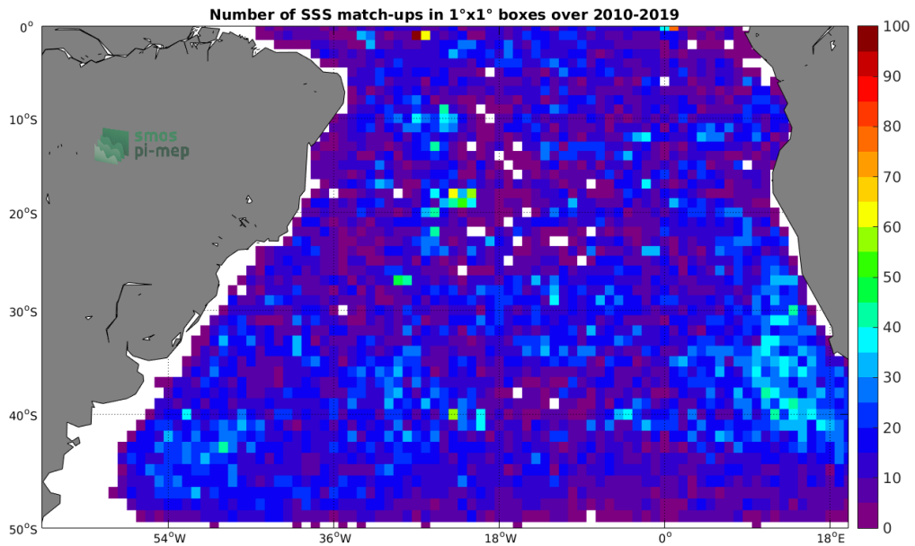
Figure 4: Number of SSS match-ups between Argo SSS and the SMOS-L2-DPGS-v662 SSS product for the South Atlantic Ocean Pi-MEP region over 1^\circ \times 1^\circ boxes and for the full satellite product period.
