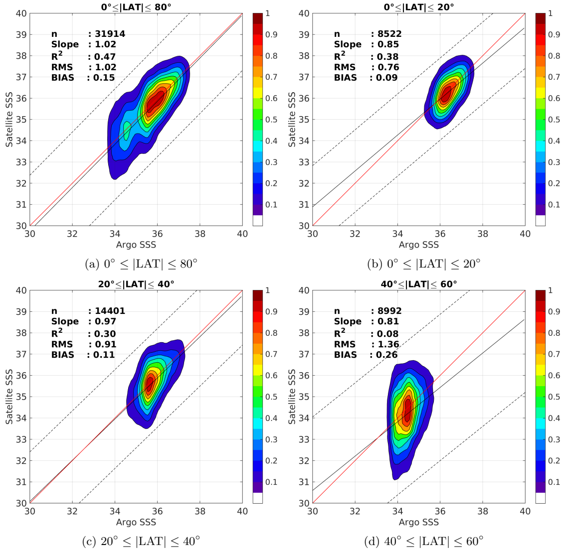
Figure 9: Contour maps of the concentration of SMOS-L2-DPGS-v662 SSS (y-axis) versus Argo SSS (x-axis) at match-up pairs for different latitude bands. For each plot, the red line shows x=y . The black thin and dashed lines indicate a linear fit through the data cloud and the \pm 95\% confidence levels, respectively. The number match-up pairs n , the slope and R^2 coefficient of the linear fit, the root mean square (RMS) and the mean bias between satellite and in situ data are indicated for each latitude band in each plots.
