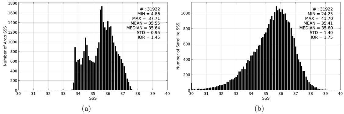
Figure 2: Histograms of SSS from Argo (a) and SMOS-L2-DPGS-v662 (b) considering all match-up pairs per bins of 0.1 over the South Atlantic Ocean Pi-MEP region and for the full satellite product period.
