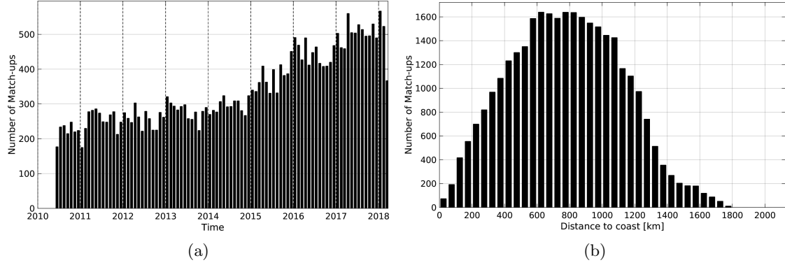
Figure 1: Number of match-ups between Argo and SMOS-L2-DPGS-v662 SSS as a function of time (a) and as function of the distance to coast (b) over the South Atlantic Ocean Pi-MEP region and for the full satellite product period.
