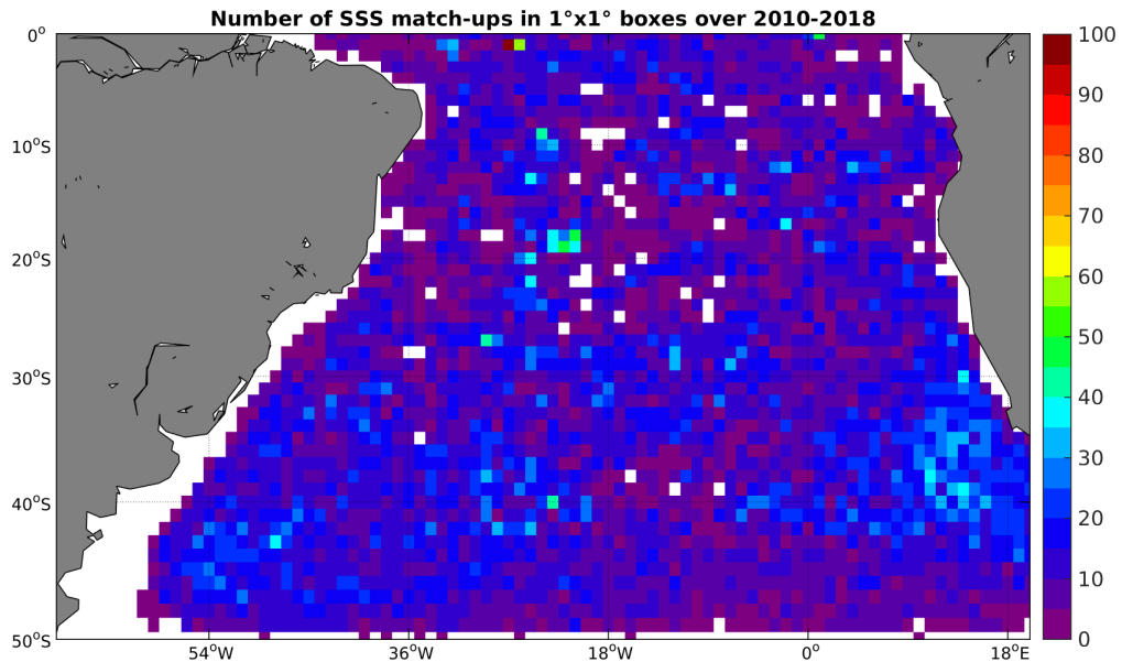
Figure 4: Number of SSS match-ups between Argo SSS and the SMOS-L2-DPGS-v662 SSS product for the South Atlantic Ocean Pi-MEP region over 1^\circ \times 1^\circ boxes and for the full satellite product period.
