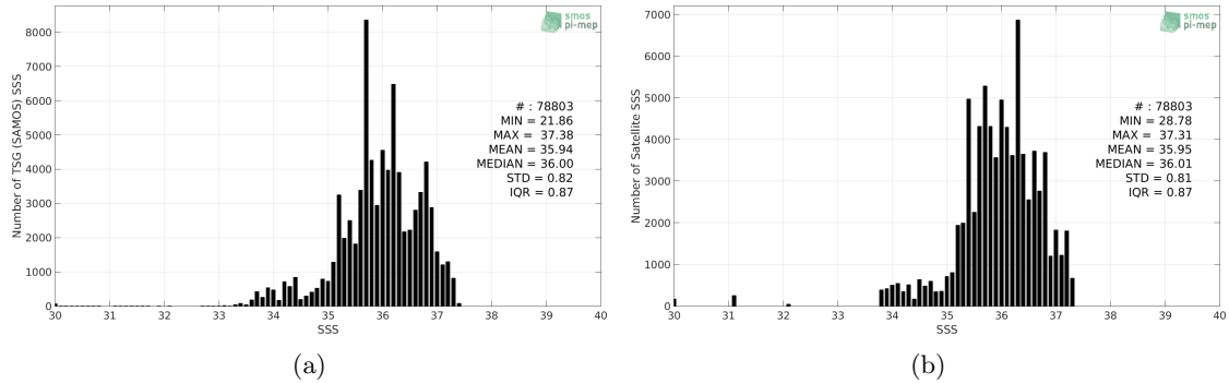
Figure 2: Histograms of SSS from TSG (SAMOS) (a) and SMAP SSS L4 OI v1 - 7day (IPRC) (b) considering all match-up pairs per bins of 0.1 over the South Atlantic Ocean Pi-MEP region and for the full satellite product period.
