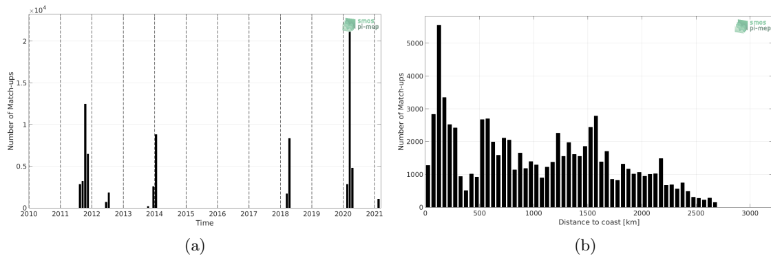
Figure 1: Number of match-ups between TSG (SAMOS) and SMAP SSS L4 OI v1 - 7day (IPRC) SSS as a function of time (a) and as function of the distance to coast (b) over the South Atlantic Ocean Pi-MEP region and for the full satellite product period.
