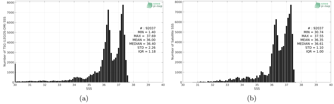
Figure 2: Histograms of SSS from TSG (LEGOS-DM) (a) and SMAP SSS L4 OI v1 - 7 Days (IPRC) (b) considering all match-up pairs per bins of 0.1 over the South Atlantic Ocean Pi-MEP region and for the full satellite product period.
