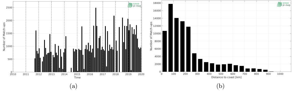
Figure 1: Number of match-ups between TSG (LEGOS-DM) and SMAP SSS L4 OI v1 - 7 Days (IPRC) SSS as a function of time (a) and as function of the distance to coast (b) over the South Atlantic Ocean Pi-MEP region and for the full satellite product period.
