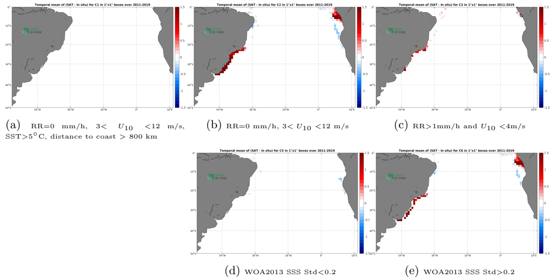
Figure 12: Temporal mean gridded over spatial boxes of size 1^\circ \times 1^\circ of \Delta SSS (SMAP SSS L4 OI v1 - 7day (IPRC) - TSG (LEGOS-DM)) for 5 different subdatasets corresponding to: RR=0 mm/h, 3 < U_{10} < 12 m/s, SST > 5^\circ C , distance to coast > 800 km (a), RR=0 mm/h, 3 < U_{10} < 12 m/s (b), RR > 1 mm/h and U_{10} < 4 m/s (c), WOA2013 SSS Std < 0.2 (d), WOA2013 SSS Std > 0.2 (e).
