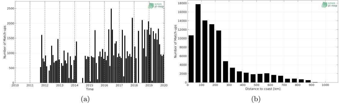
Figure 1: Number of match-ups between TSG (LEGOS-DM) and SMAP SSS L4 OI v1 - 7day (IPRC) SSS as a function of time (a) and as function of the distance to coast (b) over the South Atlantic Ocean Pi-MEP region and for the full satellite product period.
