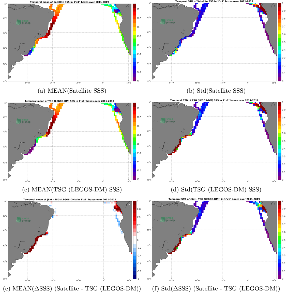
Figure 6: Temporal mean (left) and Std (right) of SSS from SMAP SSS L4 OI v1 - 7day (IPRC) (top), TSG (LEGOS-DM) (middle), and of \Delta SSS (Satellite - TSG (LEGOS-DM)). Only match-up pairs are used to generate these maps.
