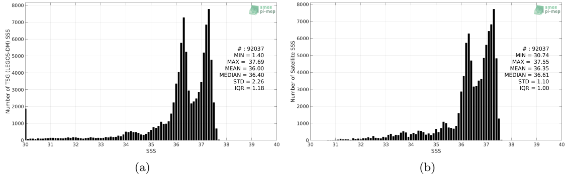
Figure 2: Histograms of SSS from TSG (LEGOS-DM) (a) and SMAP SSS L4 OI v1 - 7day (IPRC) (b) considering all match-up pairs per bins of 0.1 over the South Atlantic Ocean Pi-MEP region and for the full satellite product period.
