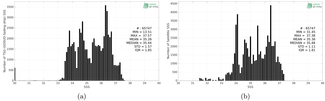
Figure 2: Histograms of SSS from TSG (GOSUD-Sailing-ship) (a) and SMAP SSS L4 OI v1 - 7 Days (IPRC) (b) considering all match-up pairs per bins of 0.1 over the South Atlantic Ocean Pi-MEP region and for the full satellite product period.
