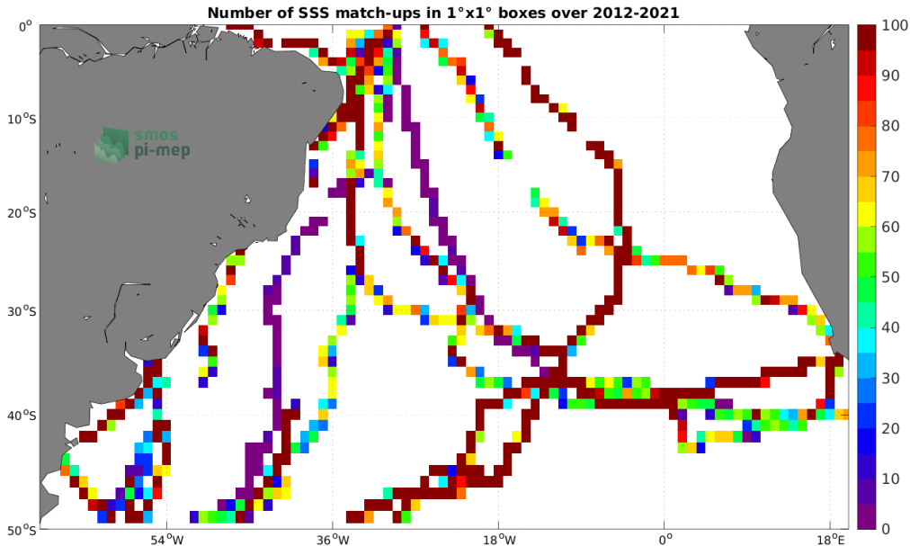
Figure 4: Number of SSS match-ups between TSG (GOSUD-Sailing-ship) SSS and the SMAP SSS L4 OI v1 - 7 Days (IPRC) SSS product for the South Atlantic Ocean Pi-MEP region over 1^\circ \times 1^\circ boxes and for the full satellite product period.
