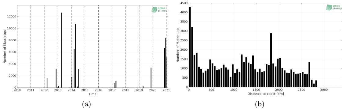
Figure 1: Number of match-ups between TSG (GOSUD-Sailing-ship) and SMAP SSS L4 OI v1 - 7 Days (IPRC) SSS as a function of time (a) and as function of the distance to coast (b) over the South Atlantic Ocean Pi-MEP region and for the full satellite product period.
