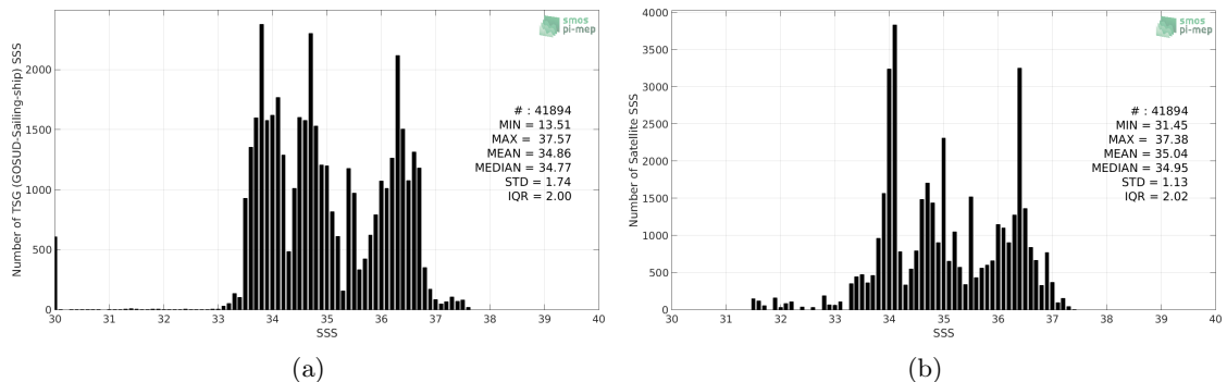
Figure 2: Histograms of SSS from TSG (GOSUD-Sailing-ship) (a) and SMAP SSS L4 OI v1 - 7day (IPRC) (b) considering all match-up pairs per bins of 0.1 over the South Atlantic Ocean Pi-MEP region and for the full satellite product period.
