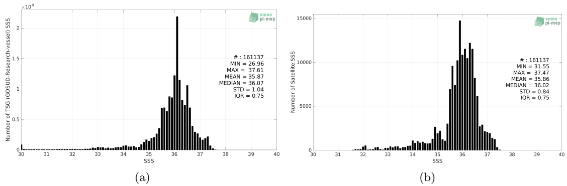
Figure 2: Histograms of SSS from TSG (GOSUD-Research-vessel) (a) and SMAP SSS L4 OI v1 - 7 Days (IPRC) (b) considering all match-up pairs per bins of 0.1 over the South Atlantic Ocean Pi-MEP region and for the full satellite product period.
