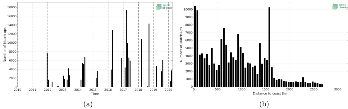
Figure 1: Number of match-ups between TSG (GOSUD-Research-vessel) and SMAP SSS L4 OI v1 - 7 Days (IPRC) SSS as a function of time (a) and as function of the distance to coast (b) over the South Atlantic Ocean Pi-MEP region and for the full satellite product period.
