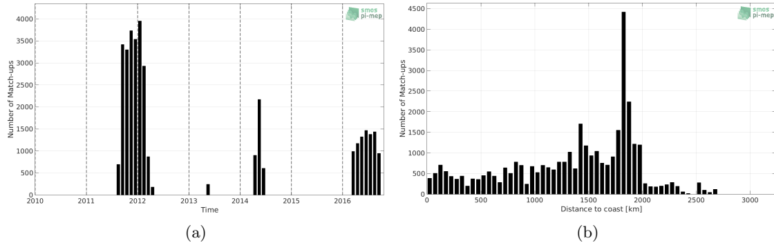
Figure 1: Number of match-ups between Surface drifters and SMAP SSS L4 OI v1 - 7 Days (IPRC) SSS as a function of time (a) and as function of the distance to coast (b) over the South Atlantic Ocean Pi-MEP region and for the full satellite product period.
