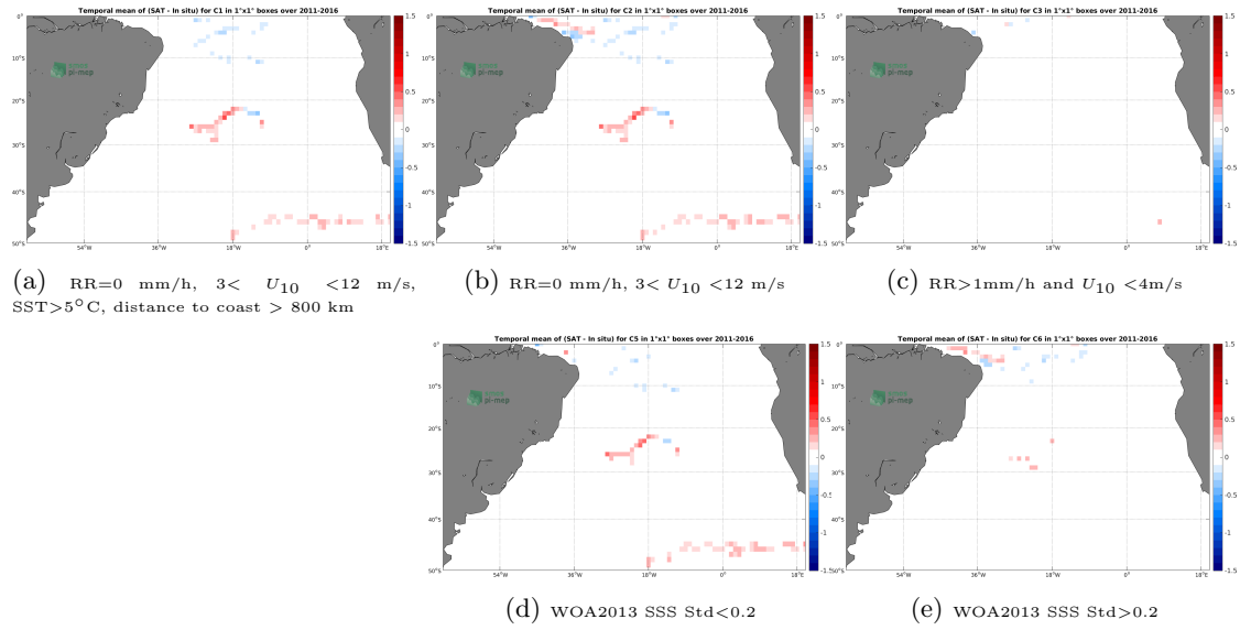
Figure 11: Temporal mean gridded over spatial boxes of size 1^\circ \times 1^\circ of \Delta SSS (SMAP SSS L4 OI v1 - 7 Days (IPRC) - Surface drifters) for 5 different subdatasets corresponding to: RR=0 mm/h, 3 < U_{10} < 12 m/s, SST > 5^\circ\text{C} , distance to coast > 800 km (a), RR=0 mm/h, 3 < U_{10} < 12 m/s (b), RR > 1 mm/h and U_{10} < 4 m/s (c), WOA2013 SSS Std < 0.2 (d), WOA2013 SSS Std > 0.2 (e).
