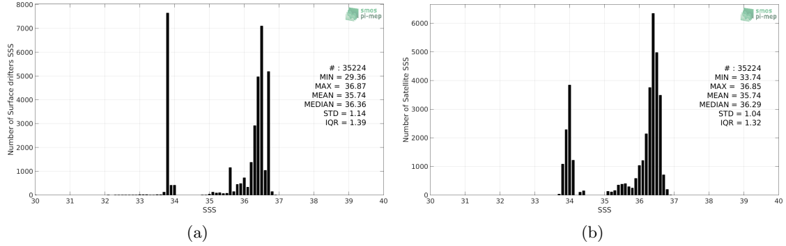
Figure 2: Histograms of SSS from Surface drifters (a) and SMAP SSS L4 OI v1 - 7 Days (IPRC) (b) considering all match-up pairs per bins of 0.1 over the South Atlantic Ocean Pi-MEP region and for the full satellite product period.
