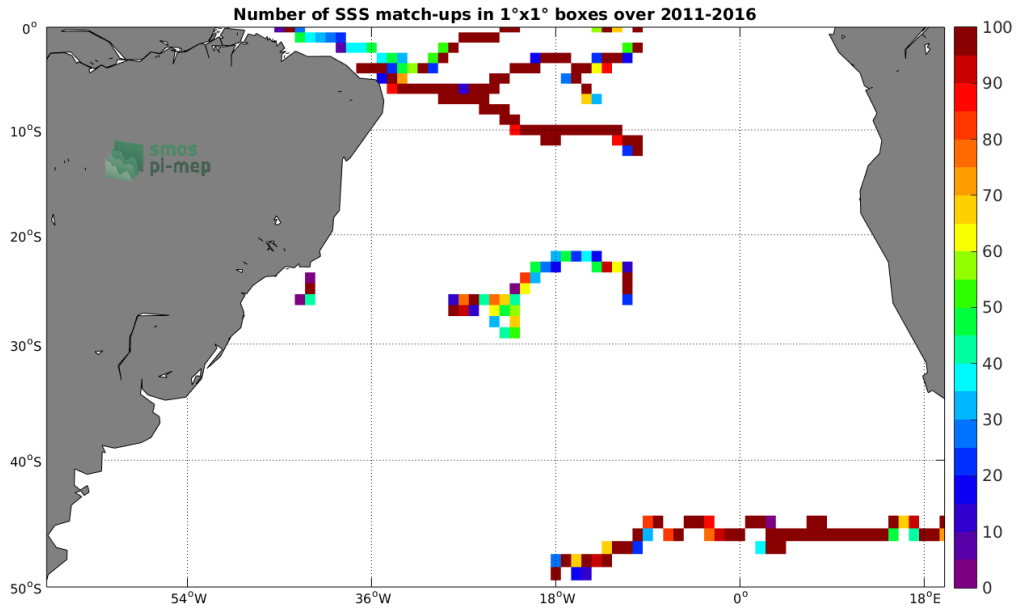
Figure 3: Number of SSS match-ups between Surface drifters SSS and the SMAP SSS L4 OI v1 - 7day (IPRC) SSS product for the South Atlantic Ocean Pi-MEP region over 1^\circ \times 1^\circ boxes and for the full satellite product period.
