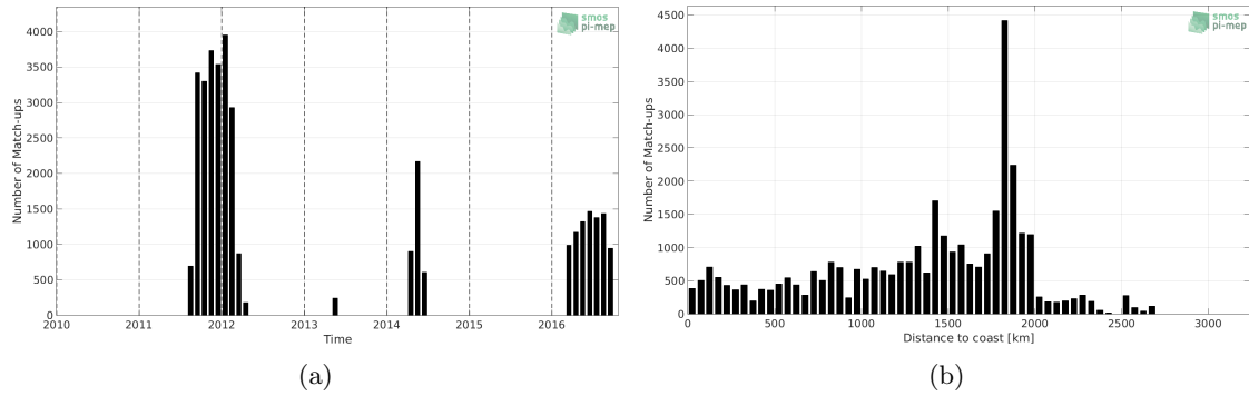
Figure 1: Number of match-ups between Surface drifters and SMAP SSS L4 OI v1 - 7day (IPRC) SSS as a function of time (a) and as function of the distance to coast (b) over the South Atlantic Ocean Pi-MEP region and for the full satellite product period.
