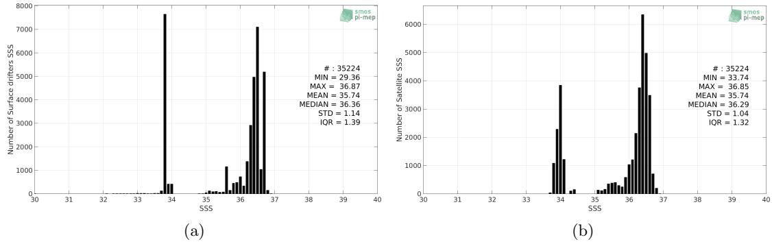
Figure 2: Histograms of SSS from Surface drifters (a) and SMAP SSS L4 OI v1 - 7day (IPRC) (b) considering all match-up pairs per bins of 0.1 over the South Atlantic Ocean Pi-MEP region and for the full satellite product period.
