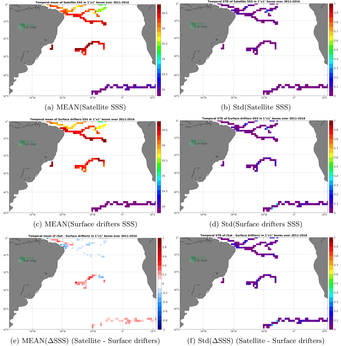
Figure 5: Temporal mean (left) and Std (right) of SSS from SMAP SSS L4 OI v1 - 7day (IPRC) (top), Surface drifters (middle), and of \Delta SSS (Satellite - Surface drifters). Only match-up pairs are used to generate these maps.
