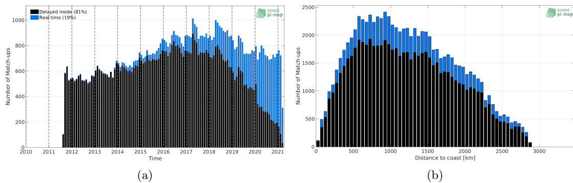
Figure 1: Number of match-ups between Argo and SMAP SSS L4 OI v1 - 7 Days (IPRC) SSS as a function of time (a) and as function of the distance to coast (b) over the South Atlantic Ocean Pi-MEP region and for the full satellite product period.
