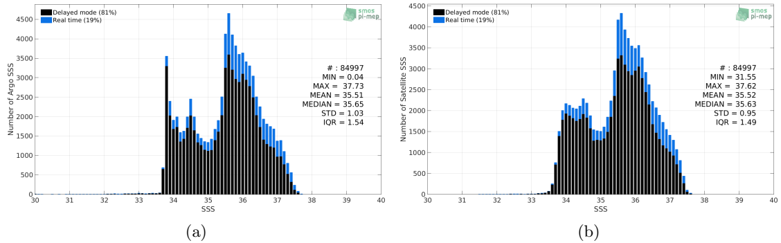
Figure 2: Histograms of SSS from Argo (a) and SMAP SSS L4 OI v1 - 7 Days (IPRC) (b) considering all match-up pairs per bins of 0.1 over the South Atlantic Ocean Pi-MEP region and for the full satellite product period.
