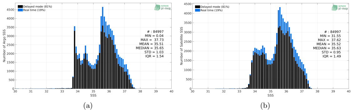
Figure 2: Histograms of SSS from Argo (a) and SMAP SSS L4 OI v1 - 7day (IPRC) (b) considering all match-up pairs per bins of 0.1 over the South Atlantic Ocean Pi-MEP region and for the full satellite product period.
