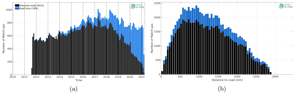
Figure 1: Number of match-ups between Argo and SMAP SSS L4 OI v1 - 7day (IPRC) SSS as a function of time (a) and as function of the distance to coast (b) over the South Atlantic Ocean Pi-MEP region and for the full satellite product period.
