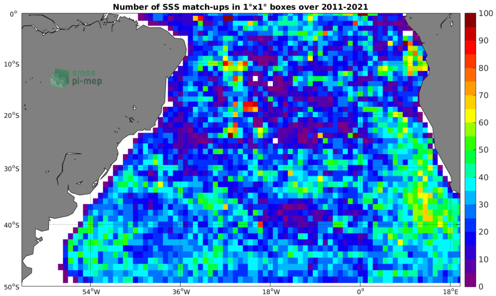
Figure 4: Number of SSS match-ups between Argo SSS and the SMAP SSS L4 OI v1 - 7day (IPRC) SSS product for the South Atlantic Ocean Pi-MEP region over 1°x1° boxes and for the full satellite product period.
