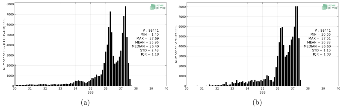
Figure 2: Histograms of SSS from TSG (LEGOS-DM) (a) and SMAP SSS L4 OI v1 - Monthly (IPRC) (b) considering all match-up pairs per bins of 0.1 over the South Atlantic Ocean Pi-MEP region and for the full satellite product period.
