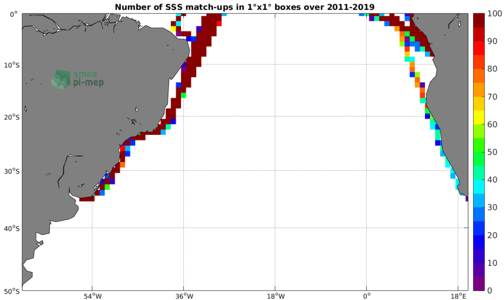
Figure 4: Number of SSS match-ups between TSG (LEGOS-DM) SSS and the SMAP SSS L4 OI v1 - Monthly (IPRC) SSS product for the South Atlantic Ocean Pi-MEP region over 1°x1° boxes and for the full satellite product period.
