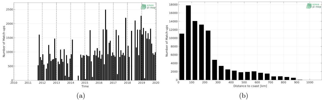
Figure 1: Number of match-ups between TSG (LEGOS-DM) and SMAP SSS L4 OI v1 - Monthly (IPRC) SSS as a function of time (a) and as function of the distance to coast (b) over the South Atlantic Ocean Pi-MEP region and for the full satellite product period.
