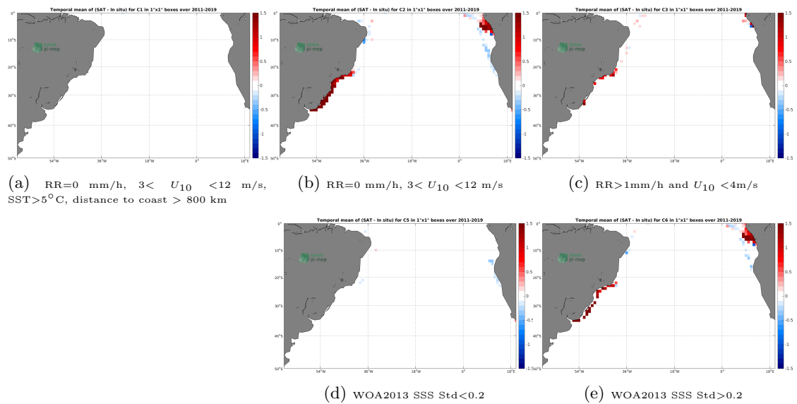
Figure 12: Temporal mean gridded over spatial boxes of size 1^\circ \times 1^\circ of \Delta SSS (SMAP SSS L4 OI v1 - Monthly (IPRC) - TSG (LEGOS-DM)) for 5 different subdatasets corresponding to: RR=0 mm/h, 3 < U_{10} < 12 m/s, SST > 5°C, distance to coast > 800 km (a), RR=0 mm/h, 3 < U_{10} < 12 m/s (b), RR > 1 mm/h and U_{10} < 4 m/s (c), WOA2013 SSS Std < 0.2 (d), WOA2013 SSS Std > 0.2 (e).
