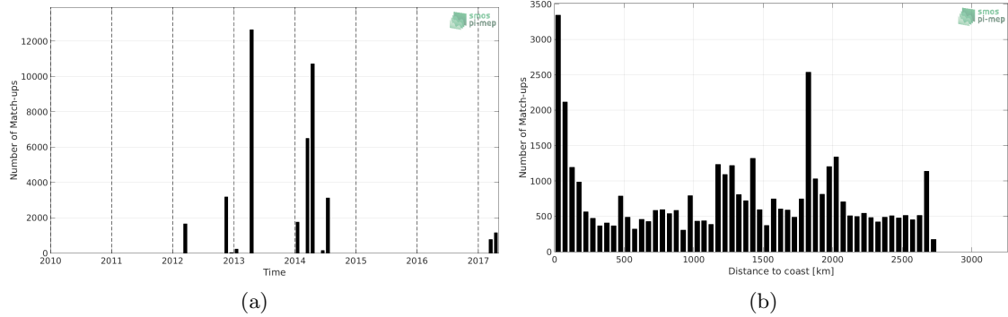
Figure 1: Number of match-ups between TSG (GOSUD-Sailing-ship) and SMAP SSS L4 OI v1 - Monthly (IPRC) SSS as a function of time (a) and as function of the distance to coast (b) over the South Atlantic Ocean Pi-MEP region and for the full satellite product period.
