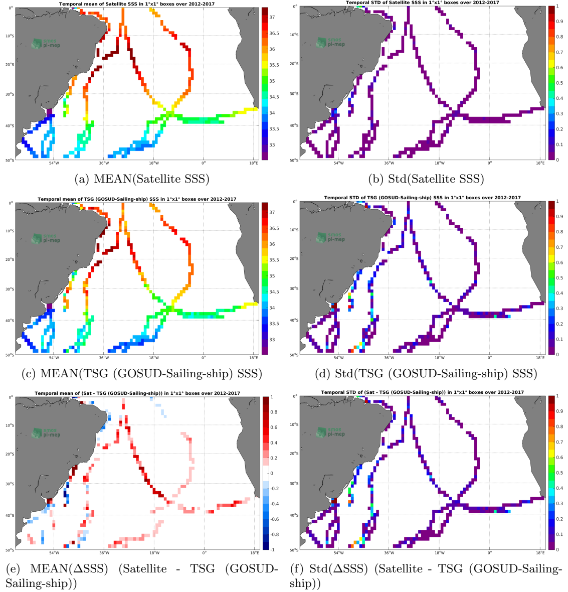
Figure 6: Temporal mean (left) and Std (right) of SSS from SMAP SSS L4 OI v1 - Monthly (IPRC) (top), TSG (GOSUD-Sailing-ship) (middle), and of \Delta SSS (Satellite - TSG (GOSUD-Sailing-ship)). Only match-up pairs are used to generate these maps.
