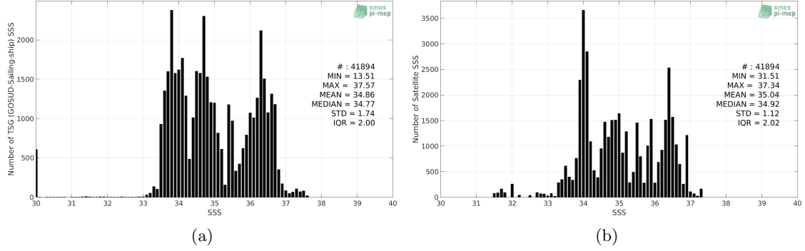
Figure 2: Histograms of SSS from TSG (GOSUD-Sailing-ship) (a) and SMAP SSS L4 OI v1 - Monthly (IPRC) (b) considering all match-up pairs per bins of 0.1 over the South Atlantic Ocean Pi-MEP region and for the full satellite product period.
