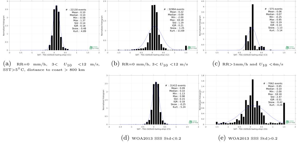
Figure 13: Normalized histogram of \Delta SSS (SMAP SSS L4 OI v1 - Monthly (IPRC) - TSG (GOSUD-Sailing-ship)) for 5 different subdatasets corresponding to: RR=0 mm/h, 3 < U_{10} < 12 m/s, SST>5°C, distance to coast > 800 km (a), RR=0 mm/h, 3 < U_{10} < 12 m/s (b), RR>1mm/h and U_{10} < 4 m/s (c), WOA2013 SSS Std<0.2 (d), WOA2013 SSS Std>0.2 (e).
