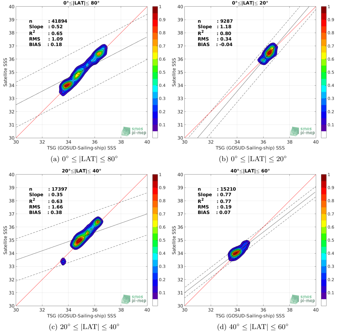
Figure 9: Contour maps of the concentration of SMAP SSS L4 OI v1 - Monthly (IPRC) SSS (y-axis) versus TSG (GOSUD-Sailing-ship) SSS (x-axis) at match-up pairs for different latitude bands. For each plot, the red line shows x=y . The black thin and dashed lines indicate a linear fit through the data cloud and the \pm 95\% confidence levels, respectively. The number match-up pairs n , the slope and R^2 coefficient of the linear fit, the root mean square (RMS) and the mean bias between satellite and in situ data are indicated for each latitude band in each plots.
