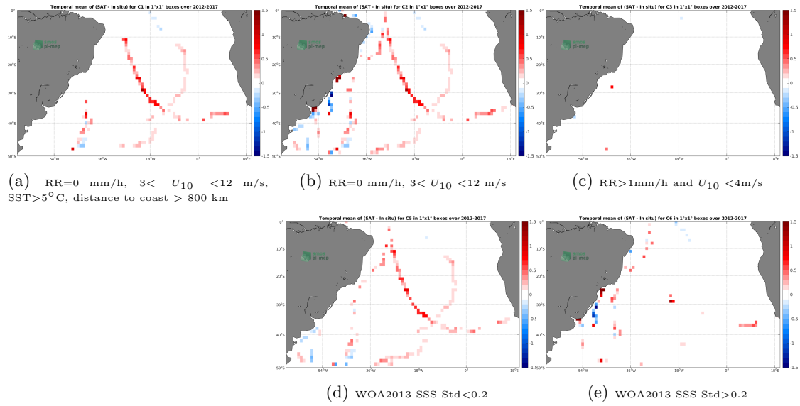
Figure 12: Temporal mean gridded over spatial boxes of size 1^\circ \times 1^\circ of \Delta SSS (SMAP SSS L4 OI v1 - Monthly (IPRC) - TSG (GOSUD-Sailing-ship)) for 5 different subdatasets corresponding to: RR=0 mm/h, 3 < U_{10} < 12 m/s, SST > 5^\circ\text{C} , distance to coast > 800 km (a), RR=0 mm/h, 3 < U_{10} < 12 m/s (b), RR > 1\text{mm/h} and U_{10} < 4\text{m/s} (c), WOA2013 SSS Std < 0.2 (d), WOA2013 SSS Std > 0.2 (e).
