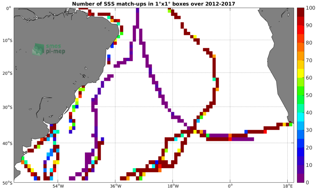
Figure 4: Number of SSS match-ups between TSG (GOSUD-Sailing-ship) SSS and the SMAP SSS L4 OI v1 - Monthly (IPRC) SSS product for the South Atlantic Ocean Pi-MEP region over 1^\circ \times 1^\circ boxes and for the full satellite product period.
