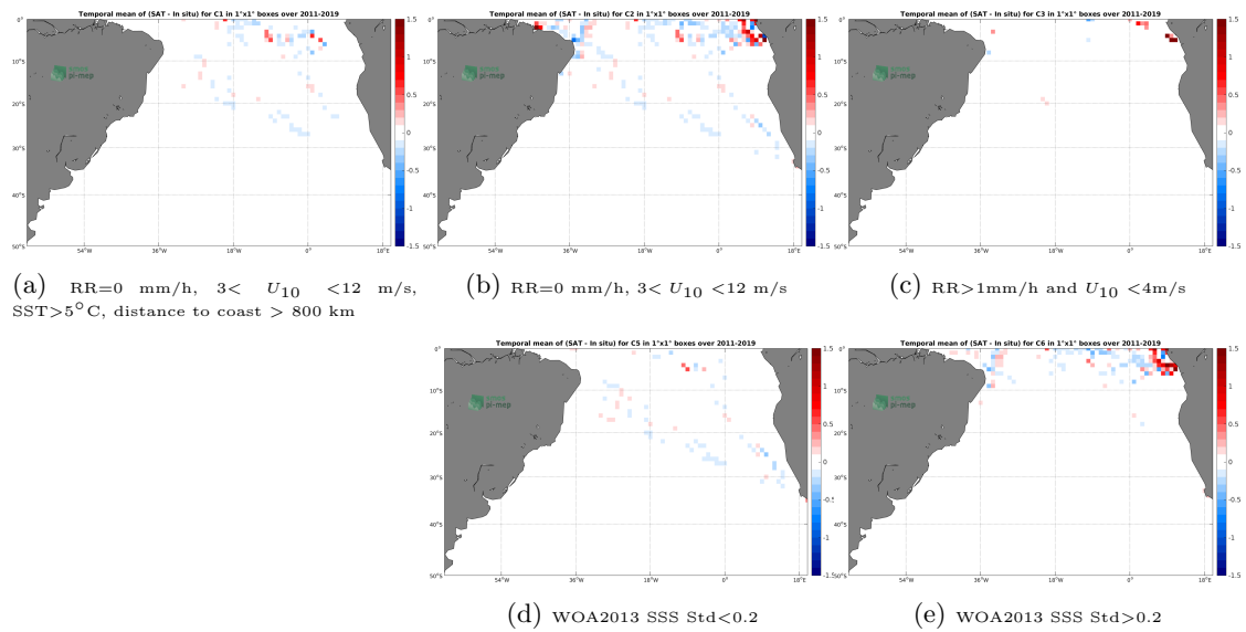
Figure 12: Temporal mean gridded over spatial boxes of size 1^\circ \times 1^\circ of \Delta\text{SSS} (SMAP SSS L4 OI v1 - Monthly (IPRC) - TSG (GOSUD-Research-vessel)) for 5 different subdatasets corresponding to: RR=0 mm/h, 3 < U_{10} < 12 m/s, SST > 5°C, distance to coast > 800 km (a), RR=0 mm/h, 3 < U_{10} < 12 m/s (b), RR > 1mm/h and U_{10} < 4 m/s (c), WOA2013 SSS Std < 0.2 (d), WOA2013 SSS Std > 0.2 (e).
