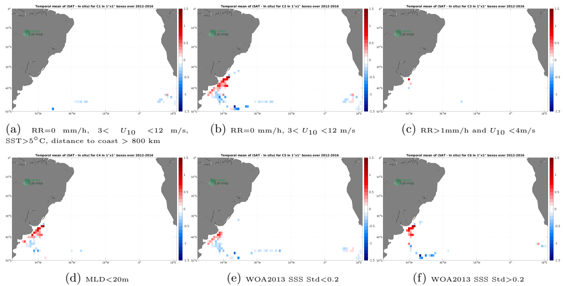
Figure 12: Temporal mean gridded over spatial boxes of size 1^\circ \times 1^\circ of \Delta SSS (SMAP SSS L4 OI v1 - Monthly (IPRC) - Marine mammals) for 6 different subdatasets corresponding to:RR=0 mm/h, 3 < U_{10} < 12 m/s, SST > 5^\circ\text{C} , distance to coast > 800 km (a), RR=0 mm/h, 3 < U_{10} < 12 m/s (b), RR > 1 mm/h and U_{10} < 4 m/s (c),MLD < 20 m (d),WOA2013 SSS Std < 0.2 (e),WOA2013 SSS Std > 0.2 (f).
