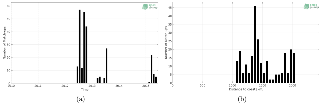
Figure 1: Number of match-ups between Marine mammals and SMAP SSS L4 OI v1 - Monthly (IPRC) SSS as a function of time (a) and as function of the distance to coast (b) over the South Atlantic Ocean Pi-MEP region and for the full satellite product period.
