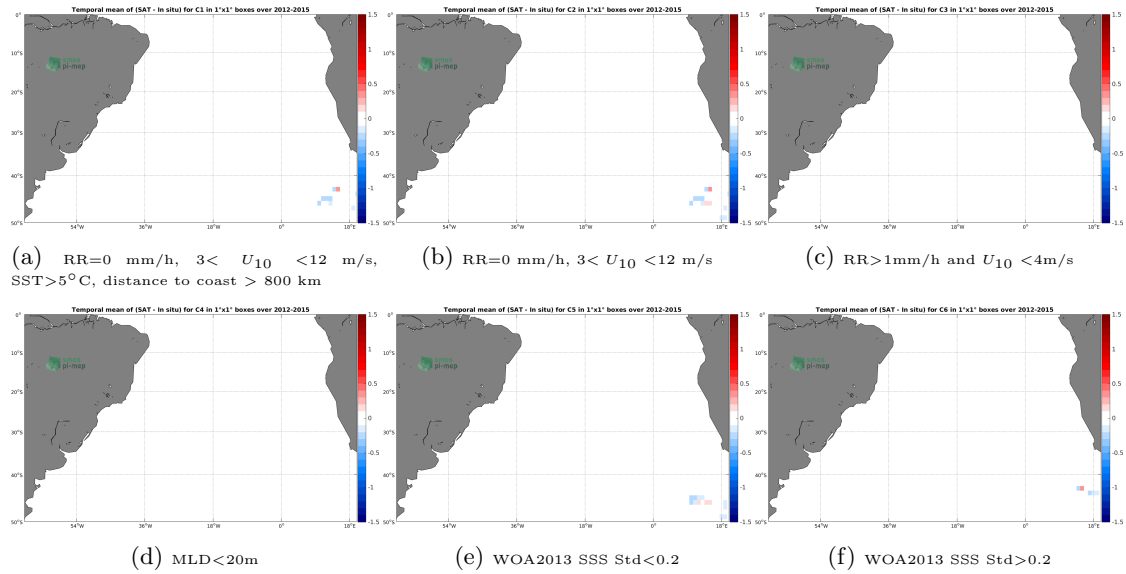
Figure 12: Temporal mean gridded over spatial boxes of size 1^{\circ}\times 1^{\circ} of \Delta\text{SSS} (SMAP SSS L4 OI v1 - Monthly (IPRC) - Marine mammals) for 6 different subdatasets corresponding to: \text{RR}=0 mm/h, 3 < U_{10} < 12 m/s, \text{SST} > 5^{\circ}\text{C} , distance to coast > 800 km (a), \text{RR}=0 mm/h, 3 < U_{10} < 12 m/s (b), \text{RR} > 1\text{mm/h} and U_{10} < 4\text{m/s} (c), \text{MLD} < 20\text{m} (d), WOA2013 SSS Std < 0.2 (e), WOA2013 SSS Std > 0.2 (f).
