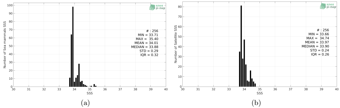
Figure 2: Histograms of SSS from Marine mammals (a) and SMAP SSS L4 OI v1 - Monthly (IPRC) (b) considering all match-up pairs per bins of 0.1 over the South Atlantic Ocean Pi-MEP region and for the full satellite product period.
