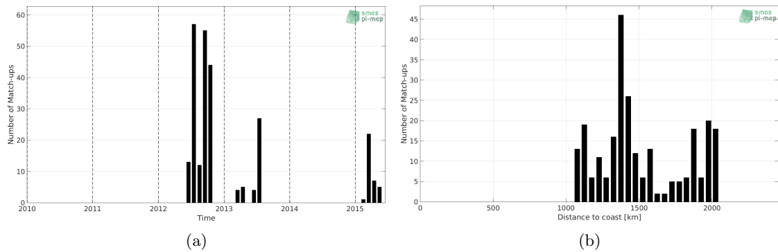
Figure 1: Number of match-ups between Sea mammals and SMAP SSS L4 OI v1 - Monthly (IPRC) SSS as a function of time (a) and as function of the distance to coast (b) over the South Atlantic Ocean Pi-MEP region and for the full satellite product period.
