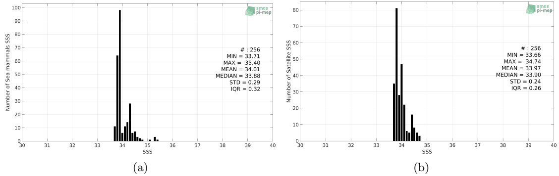
Figure 2: Histograms of SSS from Sea mammals (a) and SMAP SSS L4 OI v1 - Monthly (IPRC) (b) considering all match-up pairs per bins of 0.1 over the South Atlantic Ocean Pi-MEP region and for the full satellite product period.
