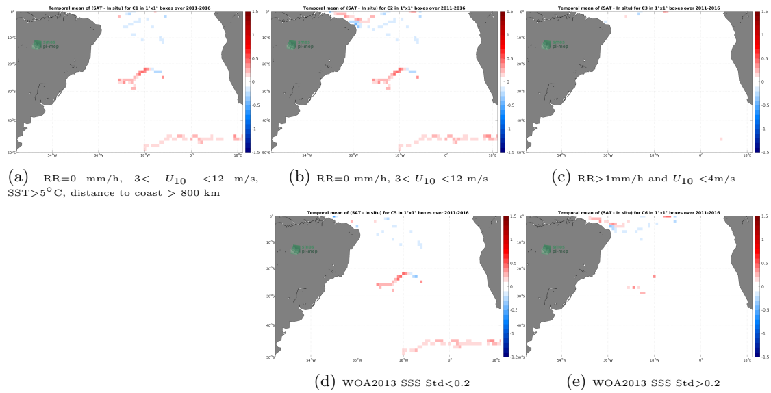
Figure 11: Temporal mean gridded over spatial boxes of size 1^\circ \times 1^\circ of \Delta SSS (SMAP SSS L4 OI v1 - Monthly (IPRC) - Surface drifters) for 5 different subdatasets corresponding to:RR=0 mm/h, 3 < U_{10} < 12 m/s, SST >5^\circ\text{C} , distance to coast > 800 km (a), RR=0 mm/h, 3 < U_{10} < 12 m/s (b), RR >1 mm/h and U_{10} < 4 m/s (c), WOA2013 SSS Std <0.2 (d), WOA2013 SSS Std >0.2 (e).
