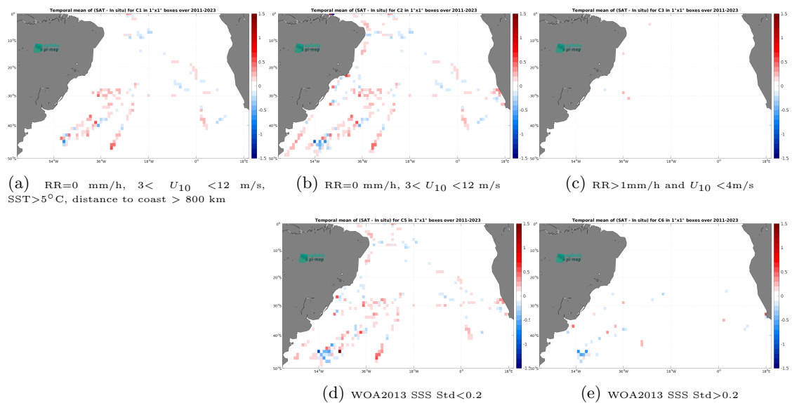
Figure 14: Temporal mean gridded over spatial boxes of size 1^\circ \times 1^\circ of \Delta\text{SSS} (SMAP SSS L4 OI v3 - Monthly (ESR) - TSG (SAMOS)) for 5 different subdatasets corresponding to:RR=0 mm/h, 3 < U_{10} < 12 m/s, SST >5^\circ\text{C} , distance to coast > 800 km (a), RR=0 mm/h, 3 < U_{10} < 12 m/s (b), RR >1 mm/h and U_{10} < 4 m/s (c), WOA2013 SSS Std <0.2 (d), WOA2013 SSS Std >0.2 (e).
