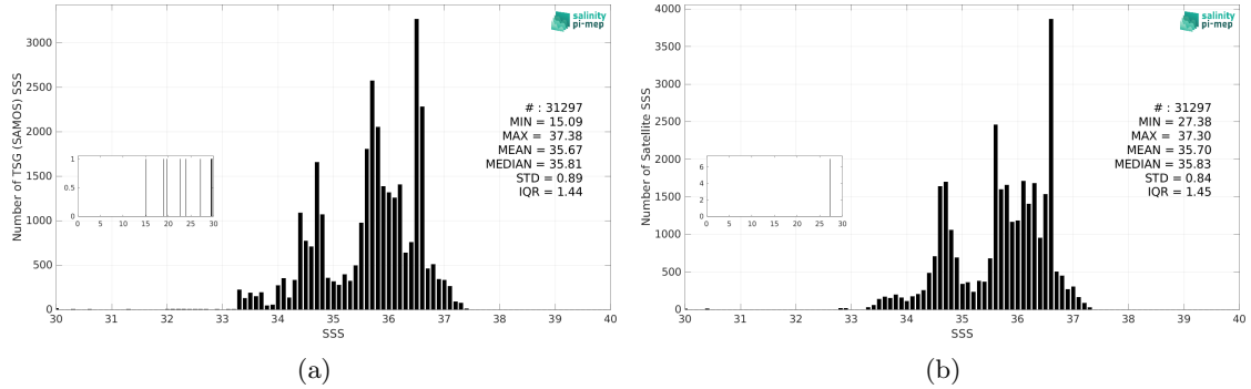
Figure 3: Histograms of SSS from TSG (SAMOS) (a) and SMAP SSS L4 OI v3 - Monthly (ESR) (b) considering all match-up pairs per bins of 0.1 over the South Atlantic Ocean Pi-MEP region and for the full satellite product period.
