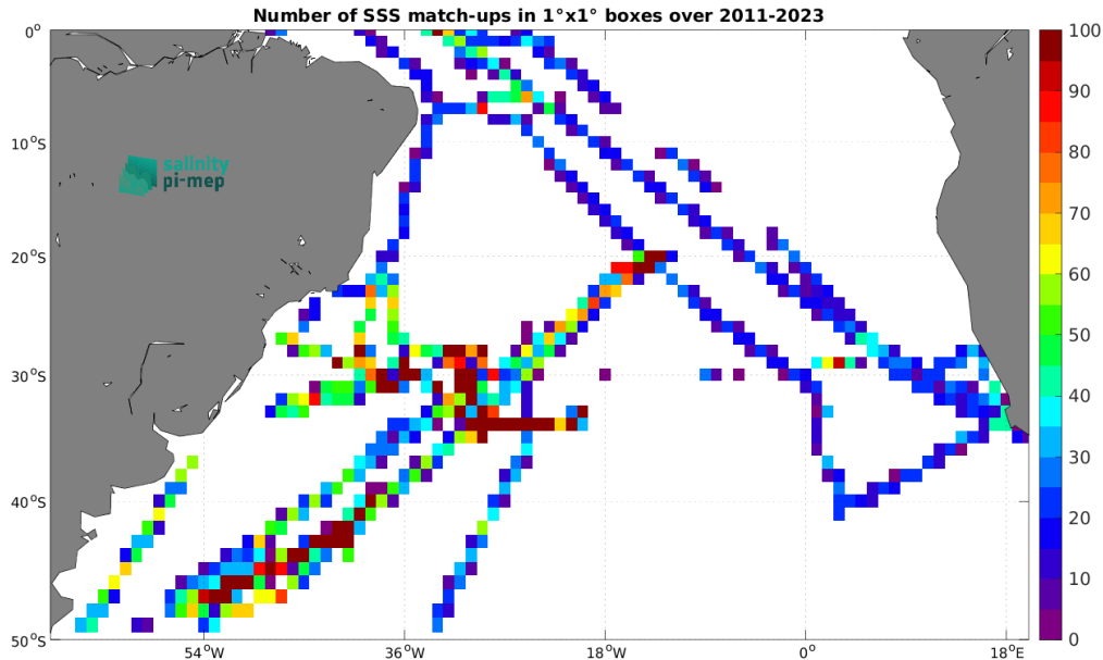
Figure 5: Number of SSS match-ups between TSG (SAMOS) SSS and the SMAP SSS L4 OI v3 - Monthly (ESR) SSS product for the South Atlantic Ocean Pi-MEP region over 1^\circ \times 1^\circ boxes and for the full satellite product period.
