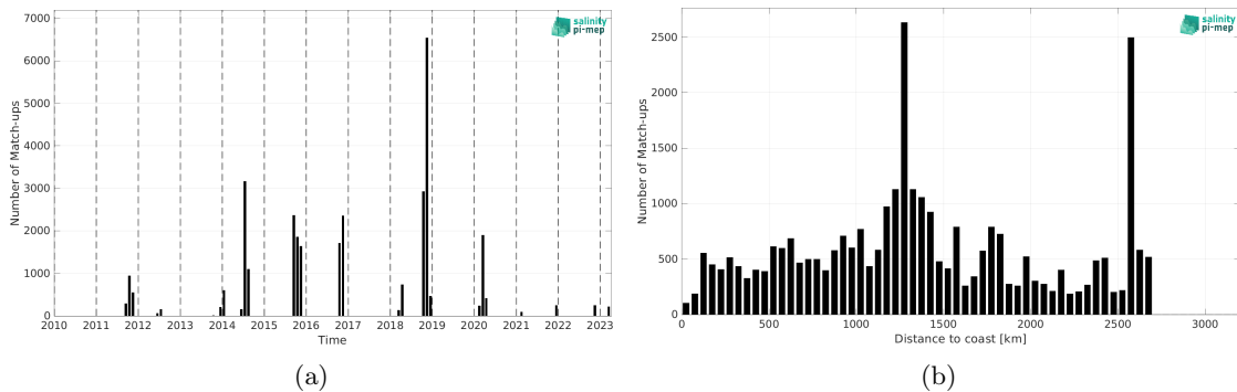
Figure 2: Number of match-ups between TSG (SAMOS) and SMAP SSS L4 OI v3 - Monthly (ESR) SSS as a function of time (a) and as function of the distance to coast (b) over the South Atlantic Ocean Pi-MEP region and for the full satellite product period.
