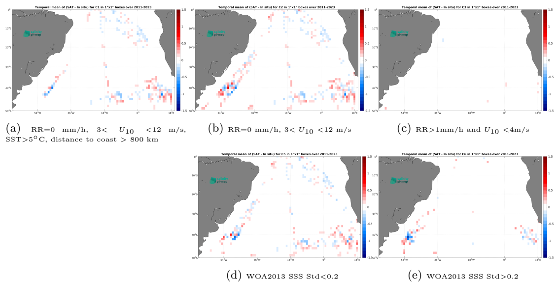
Figure 14: Temporal mean gridded over spatial boxes of size 1^\circ \times 1^\circ of \Delta\text{SSS} (SMAP SSS L4 OI v3 - Monthly (ESR) - TSG (Polarstern)) for 5 different subdatasets corresponding to:RR=0 mm/h, 3 < U_{10} < 12 m/s, SST >5^\circ\text{C} , distance to coast > 800 km (a), RR=0 mm/h, 3 < U_{10} < 12 m/s (b), RR >1 mm/h and U_{10} < 4 m/s (c), WOA2013 SSS Std <0.2 (d), WOA2013 SSS Std >0.2 (e).
