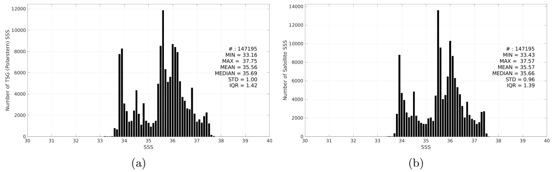
Figure 3: Histograms of SSS from TSG (Polarstern) (a) and SMAP SSS L4 OI v3 - Monthly (ESR) (b) considering all match-up pairs per bins of 0.1 over the South Atlantic Ocean Pi-MEP region and for the full satellite product period.
