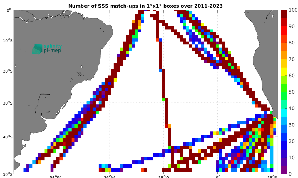
Figure 5: Number of SSS match-ups between TSG (Polarstern) SSS and the SMAP SSS L4 OI v3 - Monthly (ESR) SSS product for the South Atlantic Ocean Pi-MEP region over 1^\circ \times 1^\circ boxes and for the full satellite product period.
