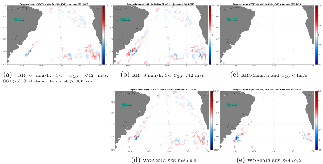
Figure 14: Temporal mean gridded over spatial boxes of size 1^\circ \times 1^\circ of \Delta SSS (SMAP SSS L4 OI v3 - Monthly (ESR) - TSG (Polarstern)) for 5 different subdatasets corresponding to:RR=0 mm/h, 3 < U_{10} < 12 m/s, SST>5°C, distance to coast > 800 km (a), RR=0 mm/h, 3 < U_{10} < 12 m/s (b), RR>1mm/h and U_{10} < 4 m/s (c), WOA2013 SSS Std<0.2 (d), WOA2013 SSS Std>0.2 (e).
