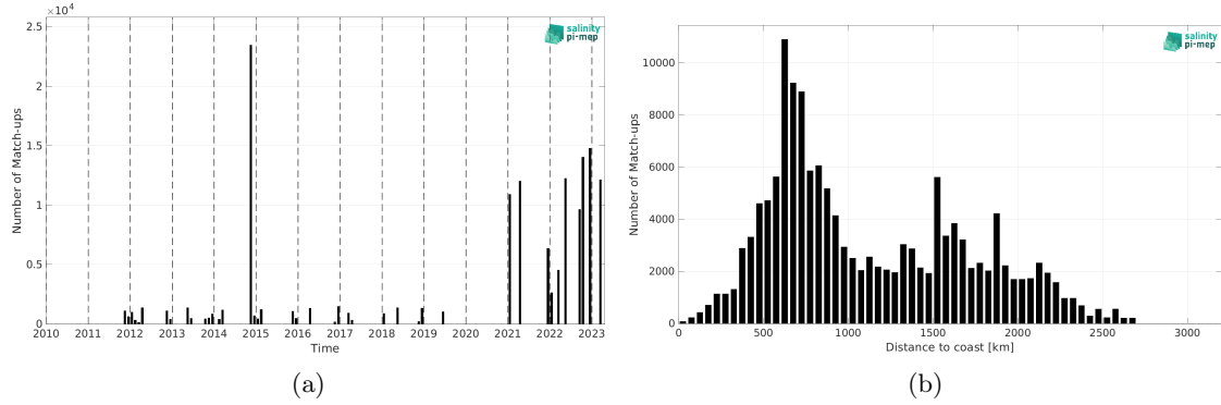
Figure 2: Number of match-ups between TSG (Polarstern) and SMAP SSS L4 OI v3 - Monthly (ESR) SSS as a function of time (a) and as function of the distance to coast (b) over the South Atlantic Ocean Pi-MEP region and for the full satellite product period.
