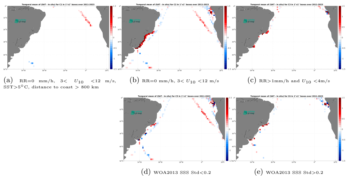
Figure 14: Temporal mean gridded over spatial boxes of size 1^\circ \times 1^\circ of \Delta\text{SSS} (SMAP SSS L4 OI v3 - Monthly (ESR) - TSG (LEGOS-DM)) for 5 different subdatasets corresponding to:RR=0 mm/h, 3 < U_{10} < 12 m/s, SST >5^\circ\text{C} , distance to coast > 800 km (a), RR=0 mm/h, 3 < U_{10} < 12 m/s (b), RR >1 mm/h and U_{10} < 4 m/s (c), WOA2013 SSS Std <0.2 (d), WOA2013 SSS Std >0.2 (e).
