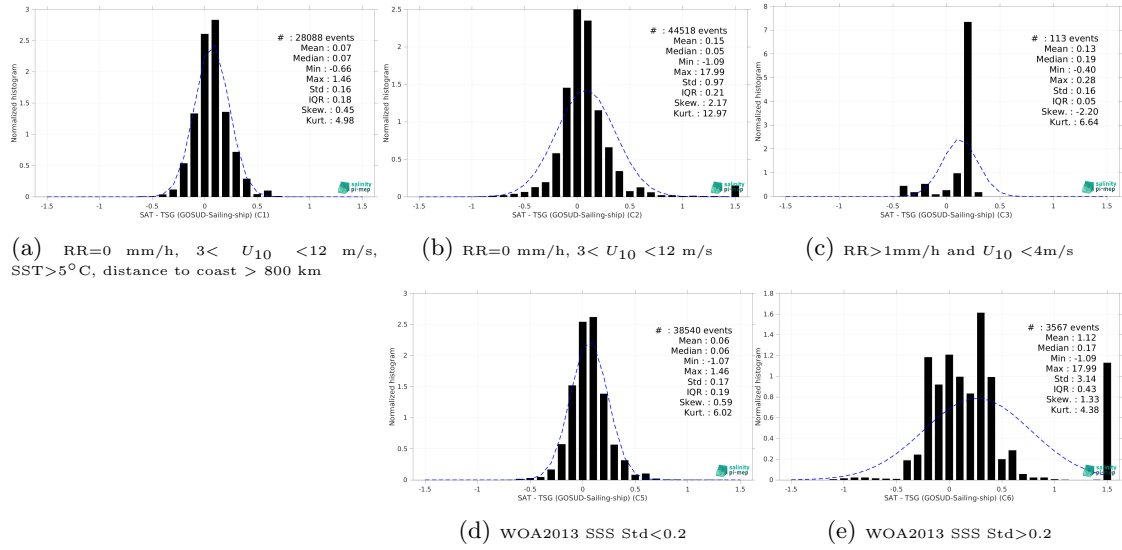
Figure 15: Normalized histogram of \Delta\text{SSS} (SMAP SSS L4 OI v3 - Monthly (ESR) - TSG (GOSUD-Sailing-ship)) for 5 different subdatasets corresponding to: RR=0 mm/h, 3 < U_{10} < 12 m/s, SST>5°C, distance to coast > 800 km (a), RR=0 mm/h, 3 < U_{10} < 12 m/s (b), RR>1mm/h and U_{10} < 4 m/s (c), WOA2013 SSS Std<0.2 (d), WOA2013 SSS Std>0.2 (e).
