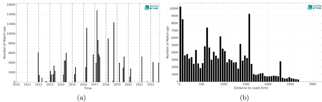
Figure 2: Number of match-ups between TSG (GOSUD-Research-vessel) and SMAP SSS L4 OI v3 - Monthly (ESR) SSS as a function of time (a) and as function of the distance to coast (b) over the South Atlantic Ocean Pi-MEP region and for the full satellite product period.
