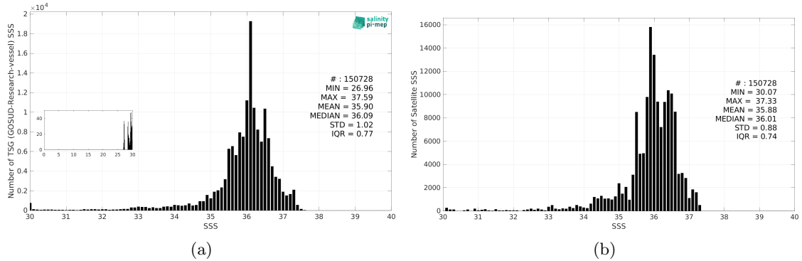
Figure 3: Histograms of SSS from TSG (GOSUD-Research-vessel) (a) and SMAP SSS L4 OI v3 - Monthly (ESR) (b) considering all match-up pairs per bins of 0.1 over the South Atlantic Ocean Pi-MEP region and for the full satellite product period.
