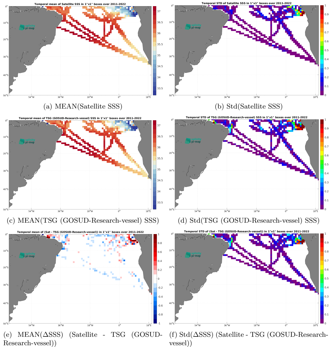
Figure 7: Temporal mean (left) and Std (right) of SSS from SMAP SSS L4 OI v3 - Monthly (ESR) (top), TSG (GOSUD-Research-vessel) (middle), and of \Delta SSS (Satellite - TSG (GOSUD-Research-vessel)). Only match-up pairs are used to generate these maps.
