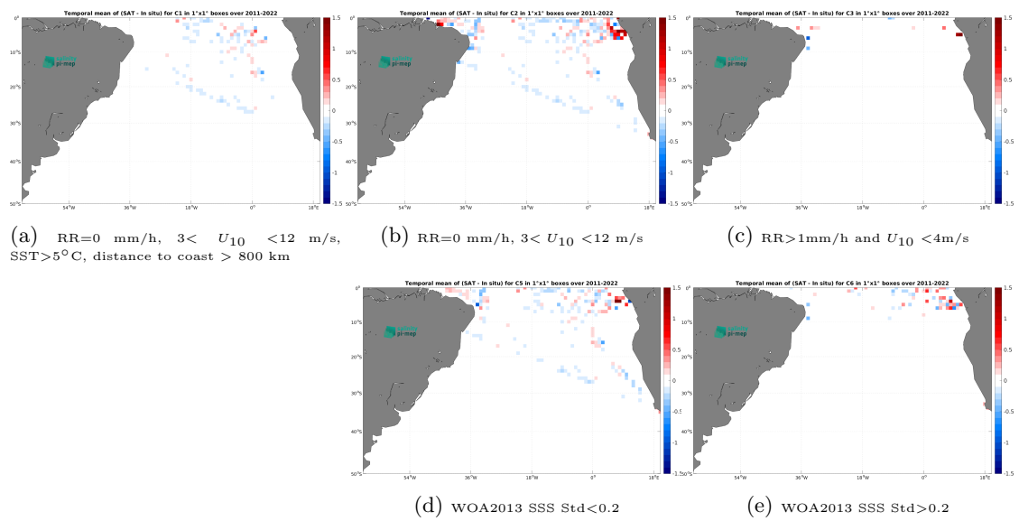
Figure 14: Temporal mean gridded over spatial boxes of size 1^\circ \times 1^\circ of \Delta SSS (SMAP SSS L4 OI v3 - Monthly (ESR) - TSG (GOSUD-Research-vessel)) for 5 different subdatasets corresponding to:RR=0 mm/h, 3 < U_{10} < 12 m/s, SST>5°C, distance to coast > 800 km (a), RR=0 mm/h, 3 < U_{10} < 12 m/s (b), RR>1mm/h and U_{10} < 4 m/s (c), WOA2013 SSS Std<0.2 (d), WOA2013 SSS Std>0.2 (e).
