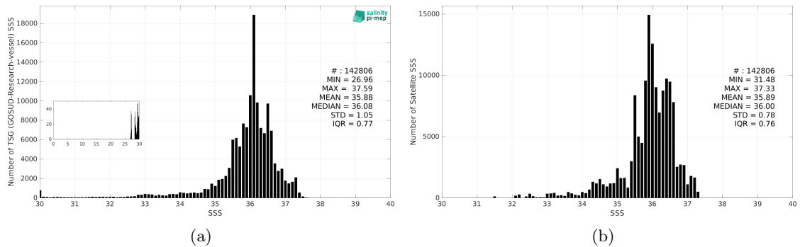
Figure 3: Histograms of SSS from TSG (GOSUD-Research-vessel) (a) and SMAP SSS L4 OI v3 - Monthly (ESR) (b) considering all match-up pairs per bins of 0.1 over the South Atlantic Ocean Pi-MEP region and for the full satellite product period.
