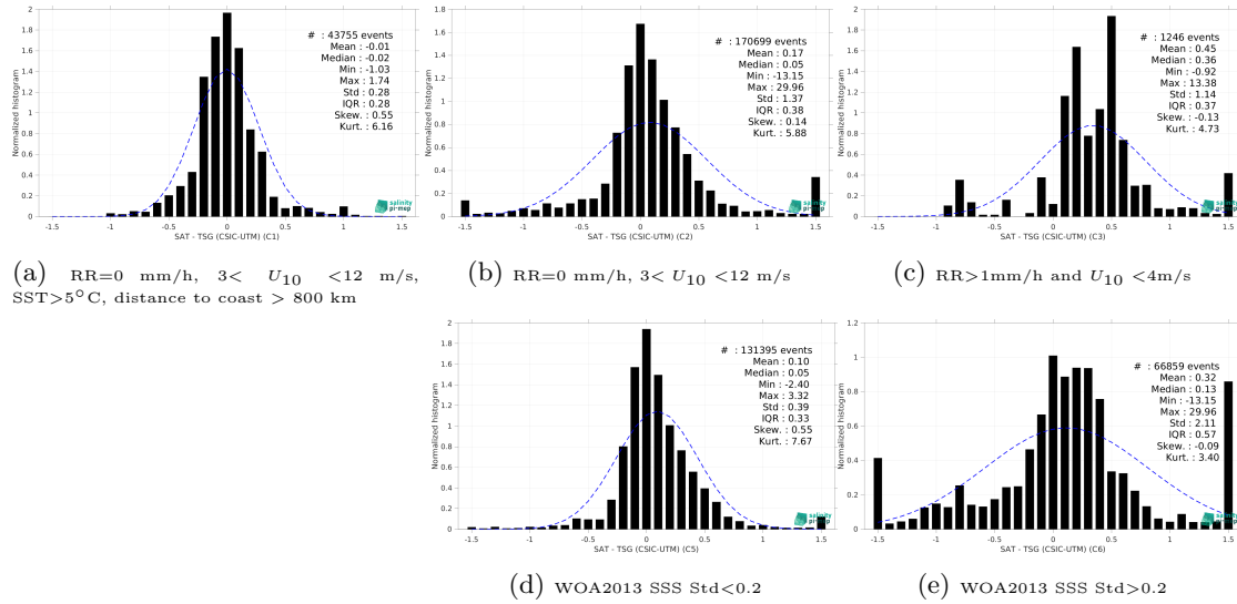
Figure 15: Normalized histogram of \Delta\text{SSS} (SMAP SSS L4 OI v3 - Monthly (ESR) - TSG (CSIC-UTM)) for 5 different subdatasets corresponding to: RR=0 mm/h, 3 < U_{10} < 12 m/s, SST>5°C, distance to coast > 800 km (a), RR=0 mm/h, 3 < U_{10} < 12 m/s (b), RR>1mm/h and U_{10} < 4 m/s (c), WOA2013 SSS Std<0.2 (d), WOA2013 SSS Std>0.2 (e).
