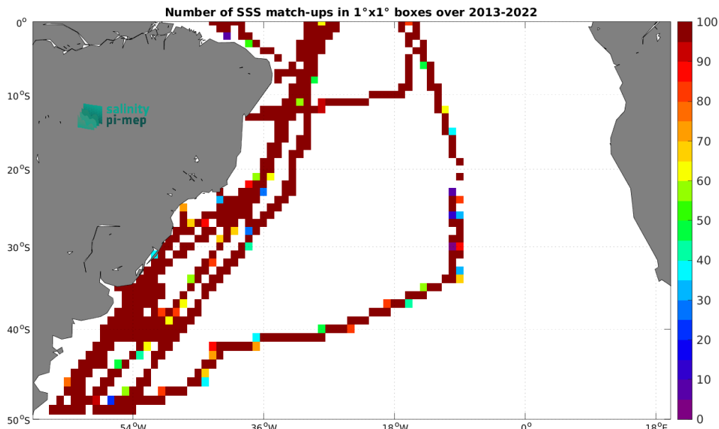
Figure 5: Number of SSS match-ups between TSG (CSIC-UTM) SSS and the SMAP SSS L4 OI v3 - Monthly (ESR) SSS product for the South Atlantic Ocean Pi-MEP region over 1^\circ \times 1^\circ boxes and for the full satellite product period.
