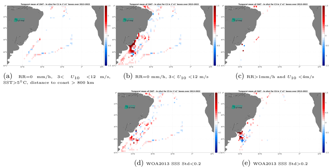
Figure 14: Temporal mean gridded over spatial boxes of size 1^\circ \times 1^\circ of \Delta\text{SSS} (SMAP SSS L4 OI v3 - Monthly (ESR) - TSG (CSIC-UTM)) for 5 different subdatasets corresponding to:RR=0 mm/h, 3 < U_{10} < 12 m/s, SST >5^\circ\text{C} , distance to coast > 800 km (a), RR=0 mm/h, 3 < U_{10} < 12 m/s (b), RR >1 mm/h and U_{10} < 4 m/s (c), WOA2013 SSS Std <0.2 (d), WOA2013 SSS Std >0.2 (e).
