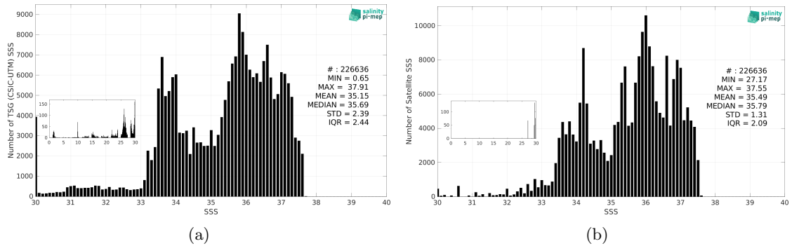
Figure 3: Histograms of SSS from TSG (CSIC-UTM) (a) and SMAP SSS L4 OI v3 - Monthly (ESR) (b) considering all match-up pairs per bins of 0.1 over the South Atlantic Ocean Pi-MEP region and for the full satellite product period.
