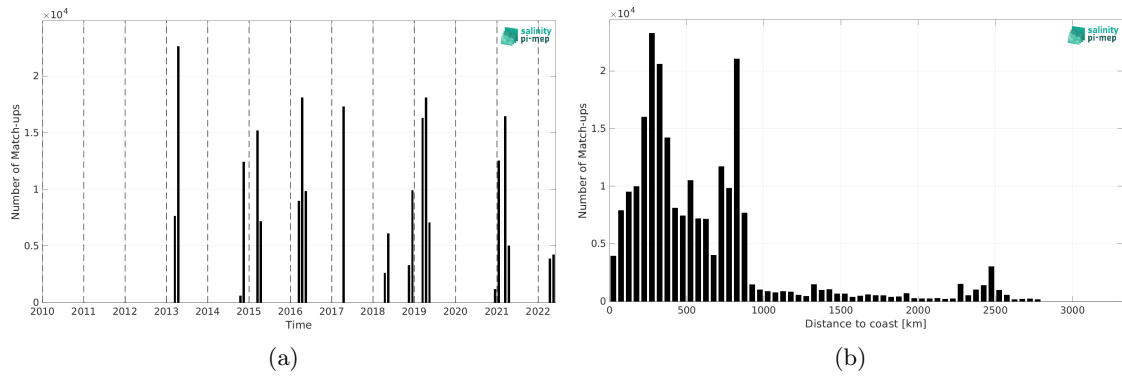
Figure 2: Number of match-ups between TSG (CSIC-UTM) and SMAP SSS L4 OI v3 - Monthly (ESR) SSS as a function of time (a) and as function of the distance to coast (b) over the South Atlantic Ocean Pi-MEP region and for the full satellite product period.
