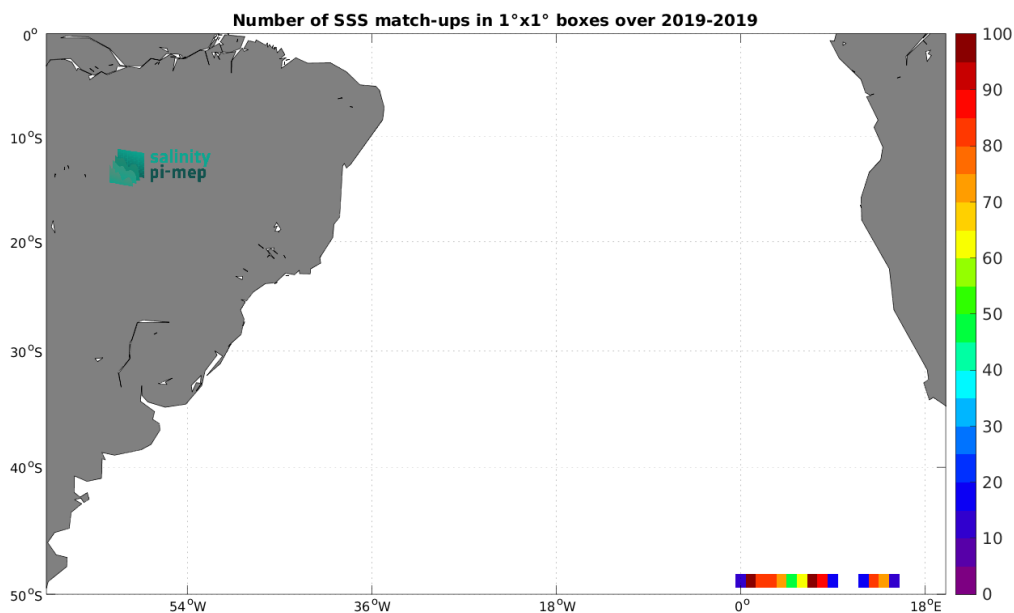
Figure 5: Number of SSS match-ups between Saildrone SSS and the SMAP SSS L4 OI v3 - Monthly (ESR) SSS product for the South Atlantic Ocean Pi-MEP region over 1^\circ \times 1^\circ boxes and for the full satellite product period.
