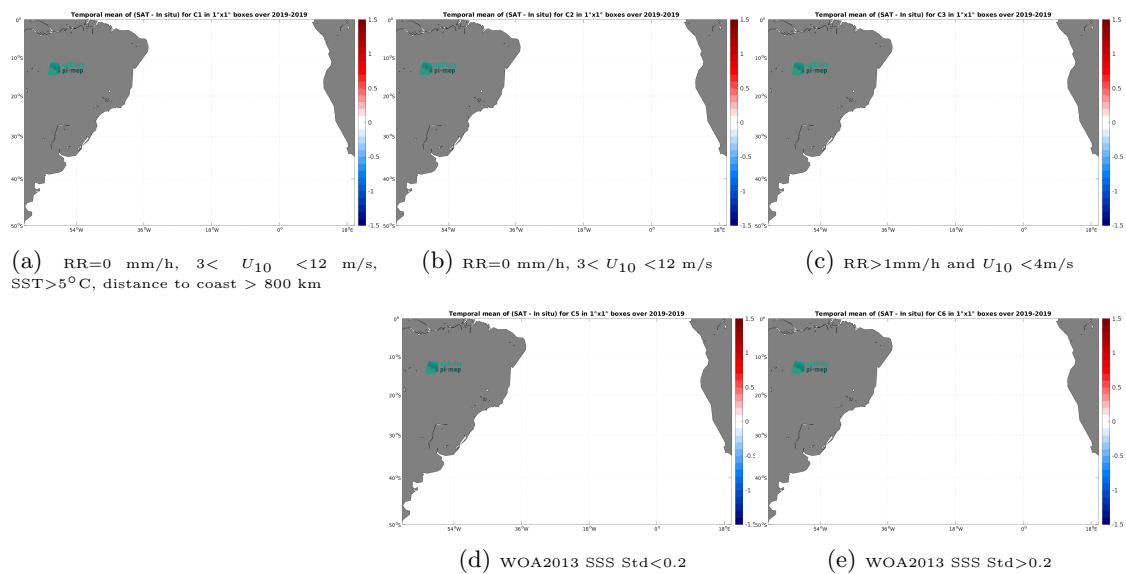
Figure 14: Temporal mean gridded over spatial boxes of size 1^\circ \times 1^\circ of \Delta SSS (SMAP SSS L4 OI v3 - Monthly (ESR) - Sairdrone) for 5 different subdatasets corresponding to:RR=0 mm/h, 3 < U_{10} < 12 m/s, SST >5^\circ\text{C} , distance to coast > 800 km (a), RR=0 mm/h, 3 < U_{10} < 12 m/s (b), RR >1 mm/h and U_{10} < 4 m/s (c), WOA2013 SSS Std <0.2 (d), WOA2013 SSS Std >0.2 (e).
