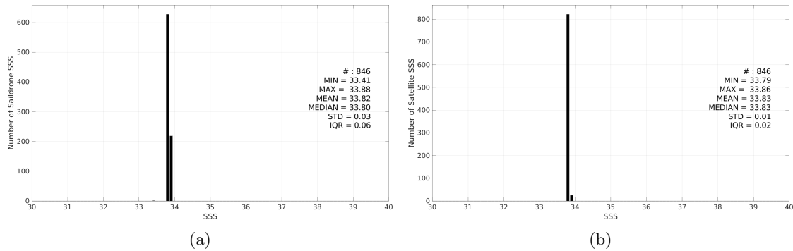
Figure 3: Histograms of SSS from Saildrone (a) and SMAP SSS L4 OI v3 - Monthly (ESR) (b) considering all match-up pairs per bins of 0.1 over the South Atlantic Ocean Pi-MEP region and for the full satellite product period.
