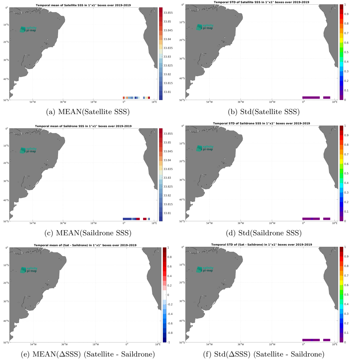
Figure 7: Temporal mean (left) and Std (right) of SSS from SMAP SSS L4 OI v3 - Monthly (ESR) (top), Saildrone (middle), and of \Delta SSS (Satellite - Saildrone). Only match-up pairs are used to generate these maps.
