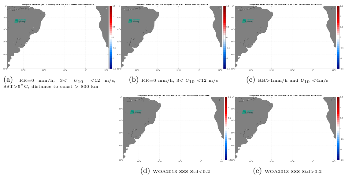
Figure 14: Temporal mean gridded over spatial boxes of size 1^\circ \times 1^\circ of \Delta SSS (SMAP SSS L4 OI v3 - Monthly (ESR) - Sairdrone) for 5 different subdatasets corresponding to:RR=0 mm/h, 3 < U_{10} < 12 m/s, SST >5^\circ\text{C} , distance to coast > 800 km (a), RR=0 mm/h, 3 < U_{10} < 12 m/s (b), RR >1 mm/h and U_{10} < 4 m/s (c), WOA2013 SSS Std <0.2 (d), WOA2013 SSS Std >0.2 (e).
